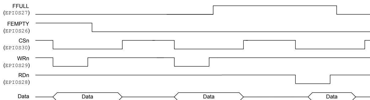
Figure 9-11. Two-Entry FIFO
