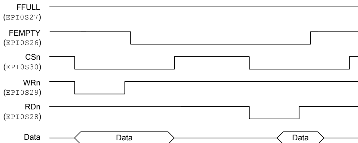
Figure 9-11. Two-Entry FIFO
