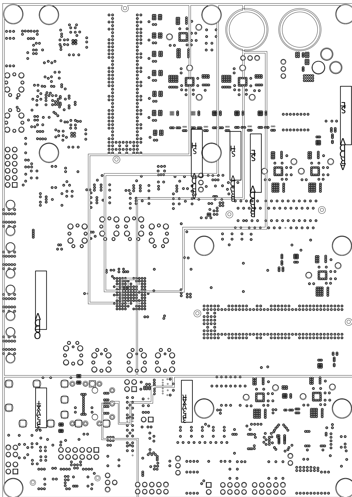
Figure 28. TLK034 EVM Layout, Internal 5-V Power (Layer 8)
