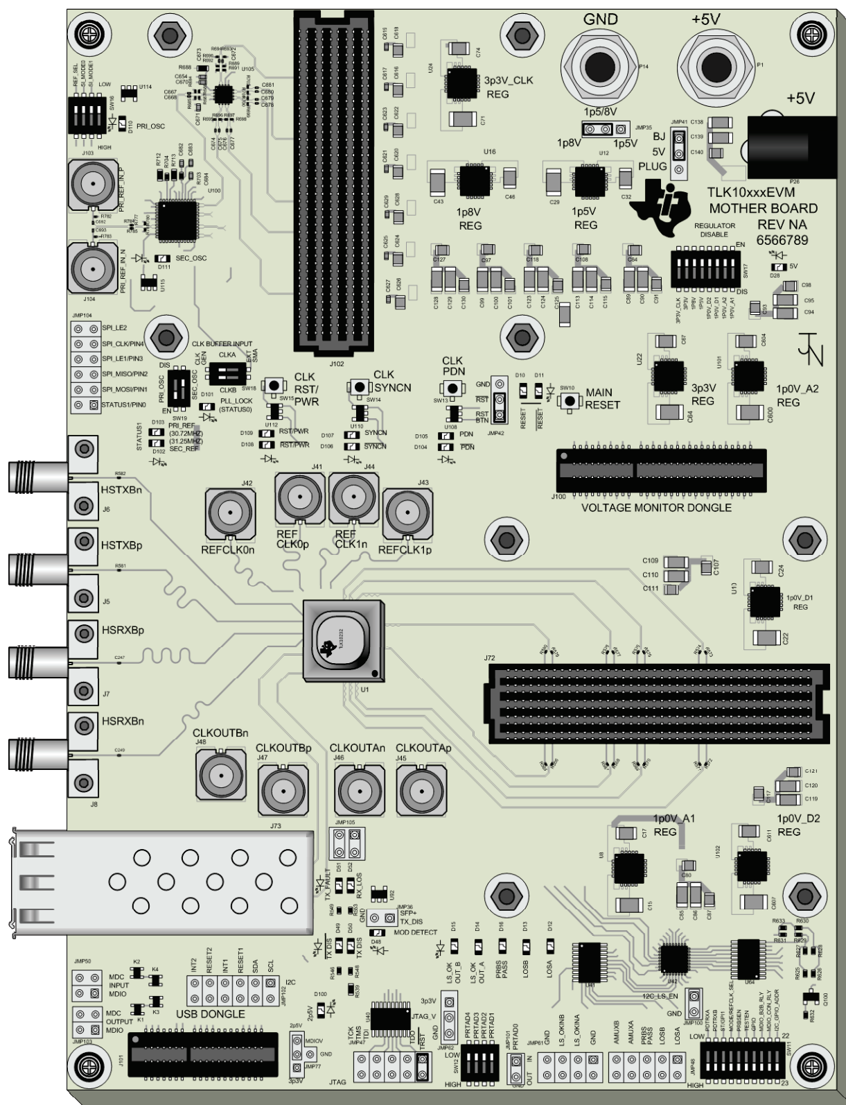
Figure 1. TLK10232 EVM Motherboard
