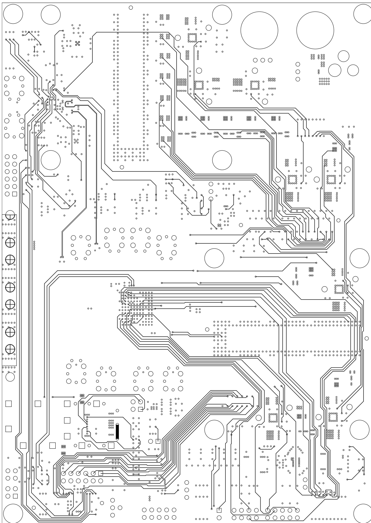
Figure 25. TLK10232 EVM Layout, Internal Signal (Layer 3)
