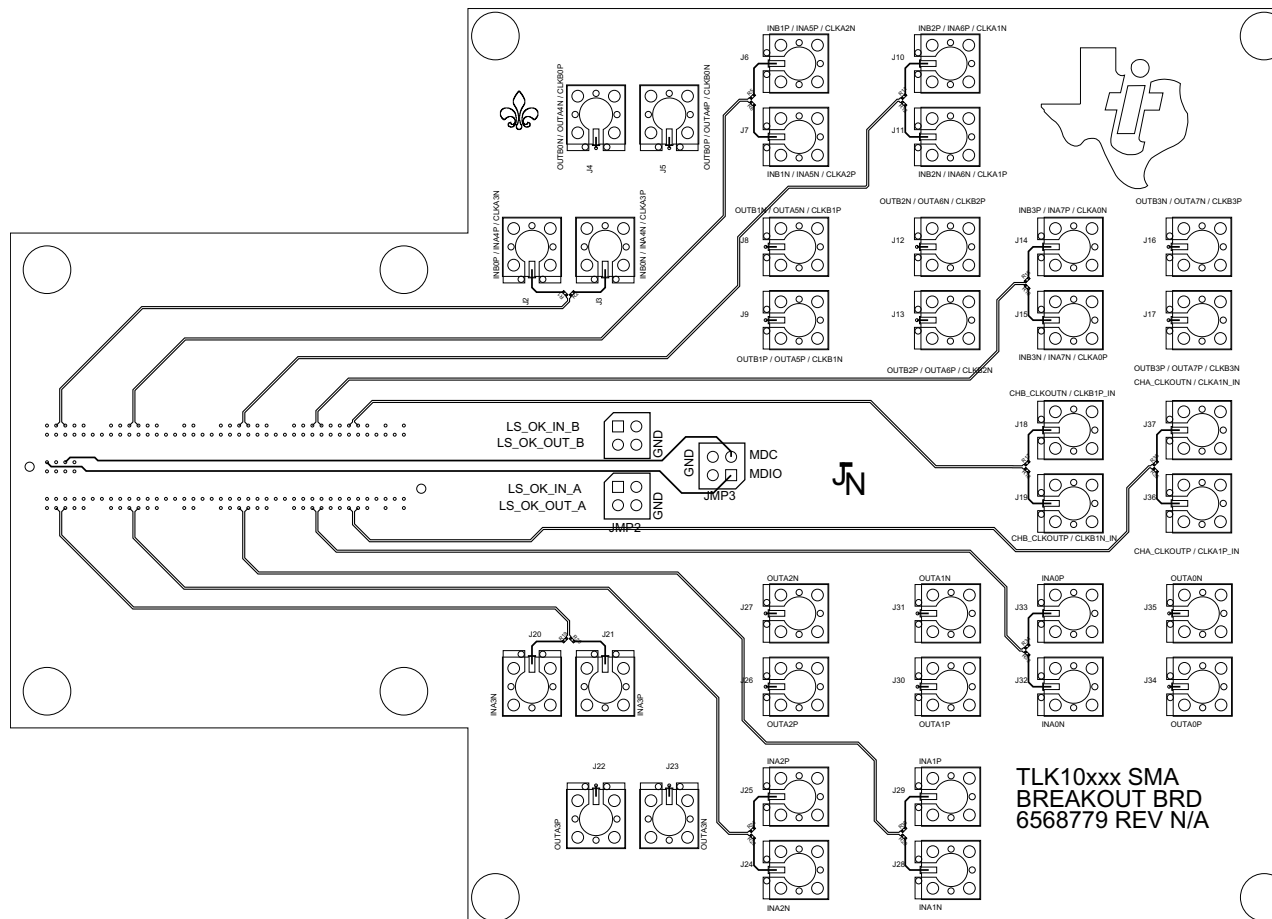
Figure 37. TLK10232 EVM SMA Breakout Board Layout, Top Signal (Layer 1)
