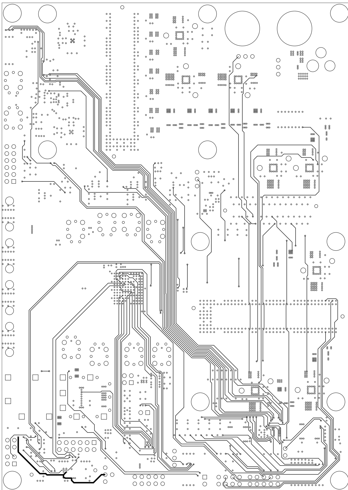
Figure 31. TLK10232 EVM Layout, Internal Signal (Layer 14)
