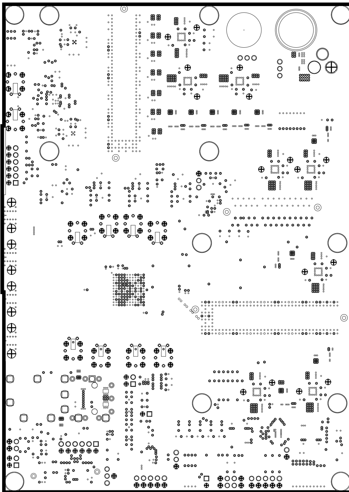
Figure 24. TLK10232 EVM Layout, Internal Ground (Layer 2)
