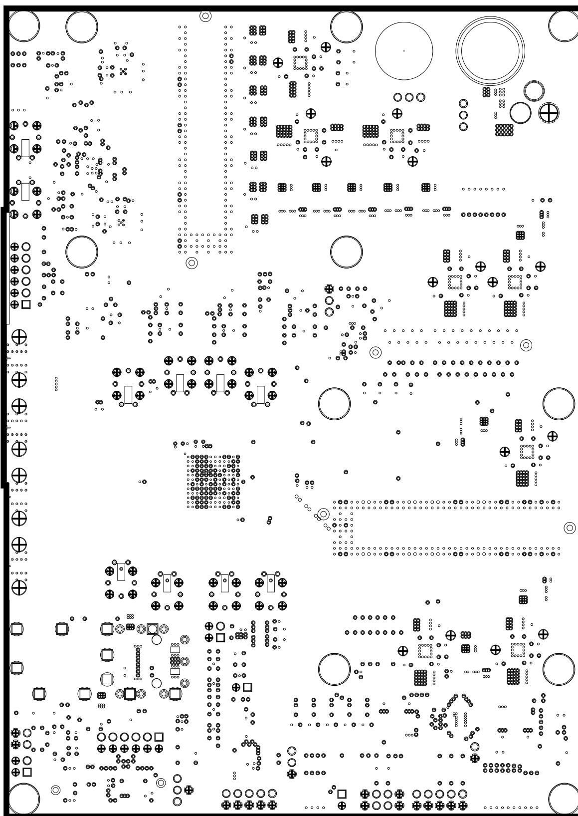
Figure 26. TLK10232 EVM Layout, Internal Ground (Layers 4, 6, 7, 9, 11, 13, 15)
