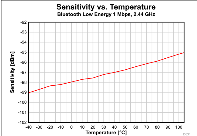
Figure 7-12. Sensitivity vs. Temperature (Bluetooth Low Energy 1 Mbps, 2.44 GHz)
