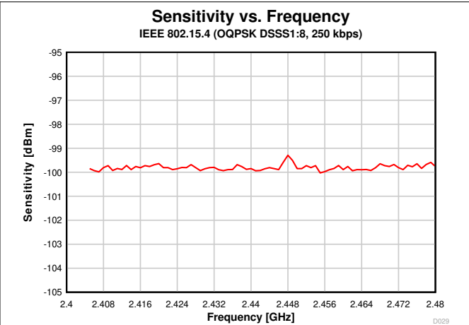
Figure 7-11. Sensitivity vs. Frequency (250 kbps, 2.44 GHz)
