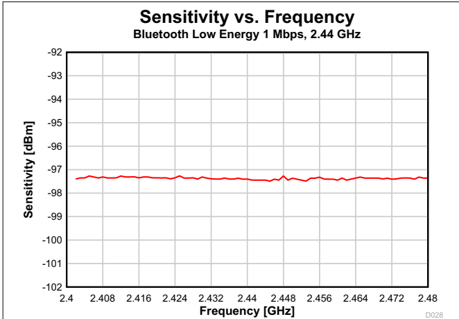
Figure 7-10. Sensitivity vs. Frequency (Bluetooth Low Energy 1 Mbps, 2.44 GHz)
