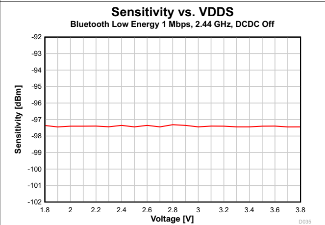
Figure 7-15. Sensitivity vs. Supply Voltage (VDD5) (Bluetooth Low Energy 1 Mbps, 2.44 GHz, DCDC Off)
