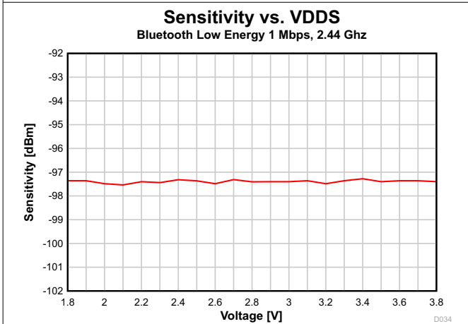
Figure 7-14. Sensitivity vs. Supply Voltage (VDD5) (Bluetooth Low Energy 1 Mbps, 2.44 GHz)
