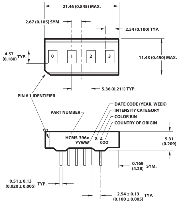
Figure 3: HCMS-396X Package Dimensions
