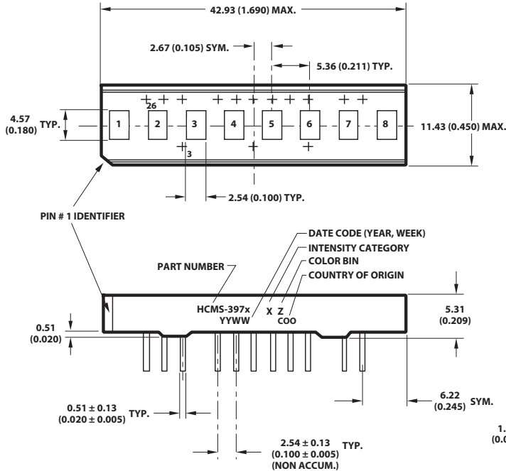
Figure 4: HCMS-397X Package Dimensions
