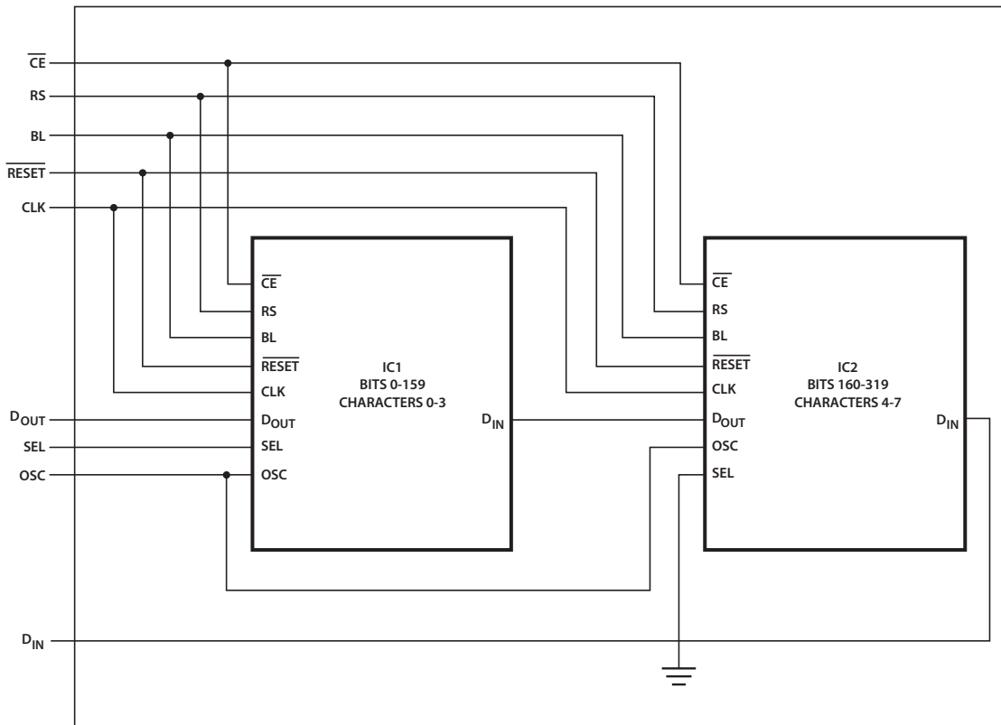
Figure 9: Cascaded ICs
