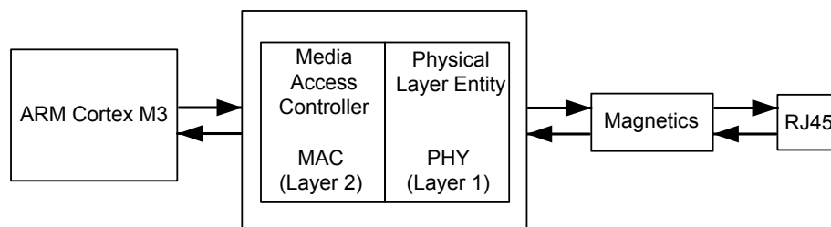
Figure 16-1. Ethernet Controller
