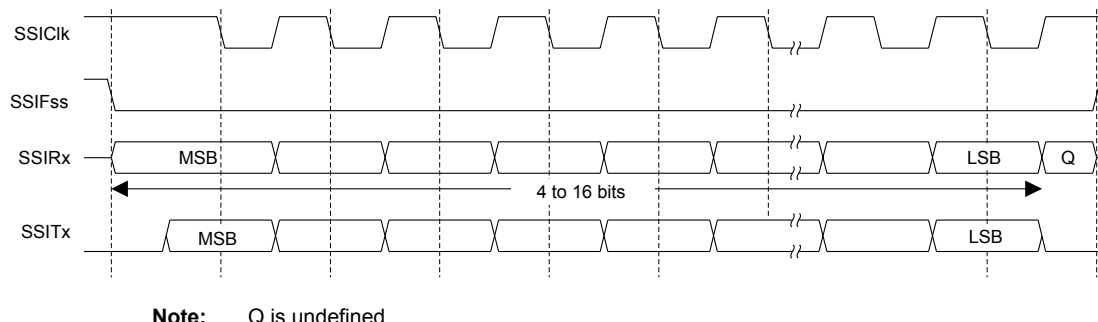
Figure 14-8. Freescale SPI Frame Format (Continuous Transfer) with SPO=1 and SPH=0
