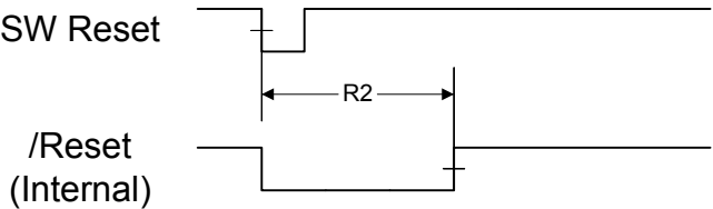
Figure 21-8. Software Reset Timing
