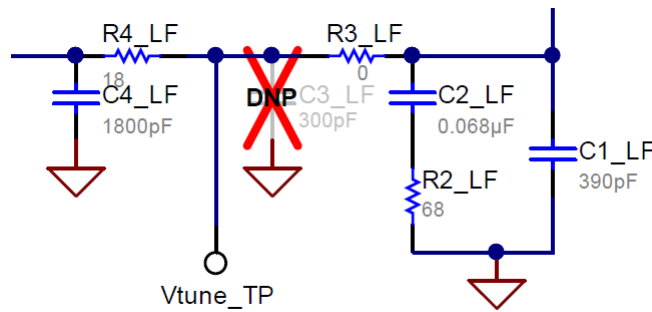
Figure 4-1. Current Loop Filter Configuration
