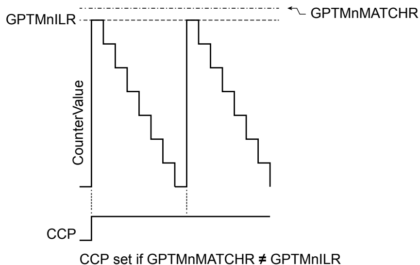
Figure 11-6. CCP Output, GPTMTnMATCHHR > GPTMTnILR
