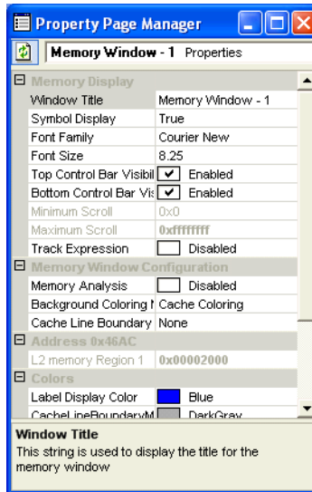
Figure 5-11. Property Window
