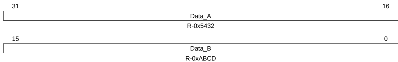
Figure 23-30. Global Static Number 0 (GSN0) [offset_TU = 00h]
