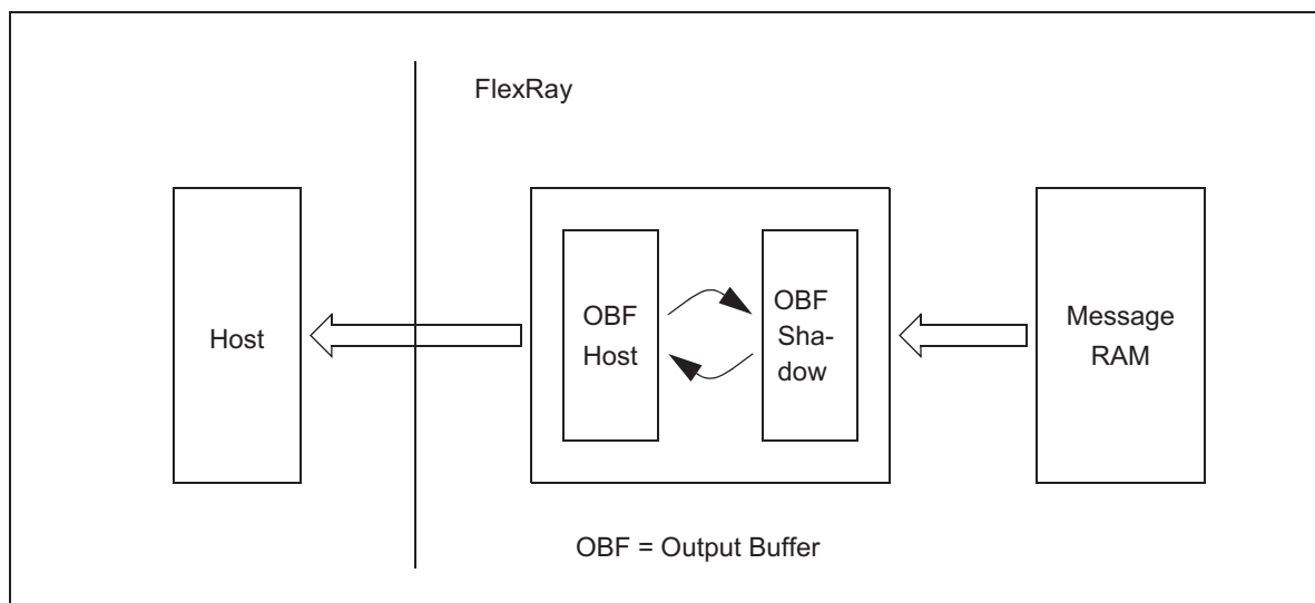
Figure 23-20. Double Buffer Structure Output Buffer
