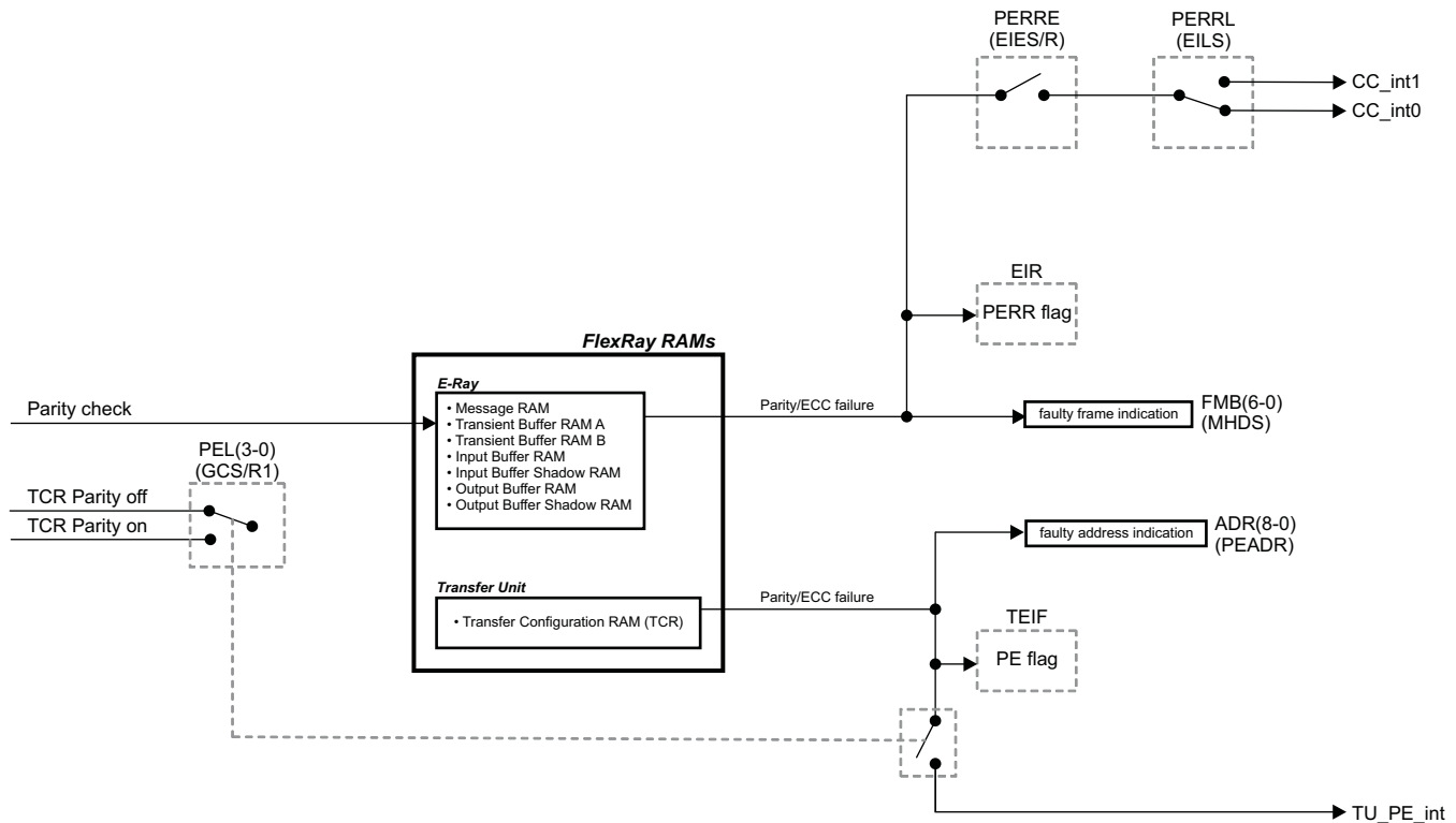
Figure 23-26. Parity Structure
