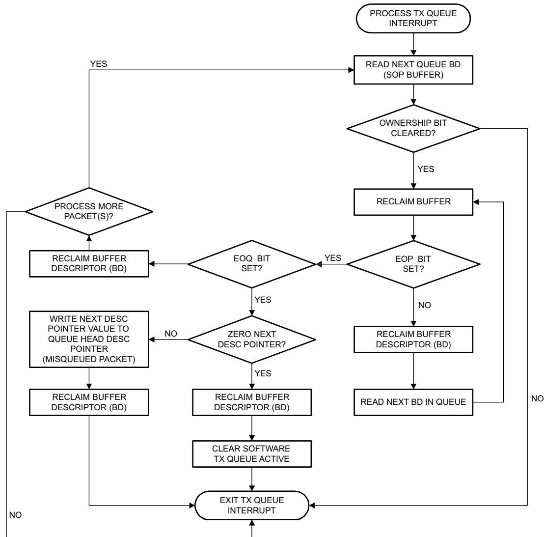
Figure 29-9. Transmit Queue Interrupt Processing Flow Chart
