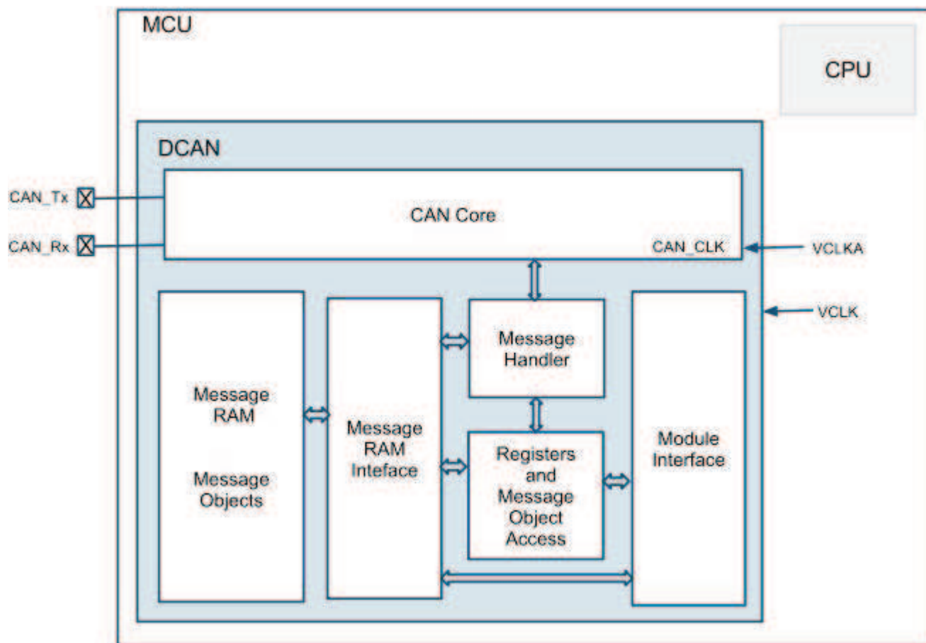
Figure 24-1. Block Diagram
