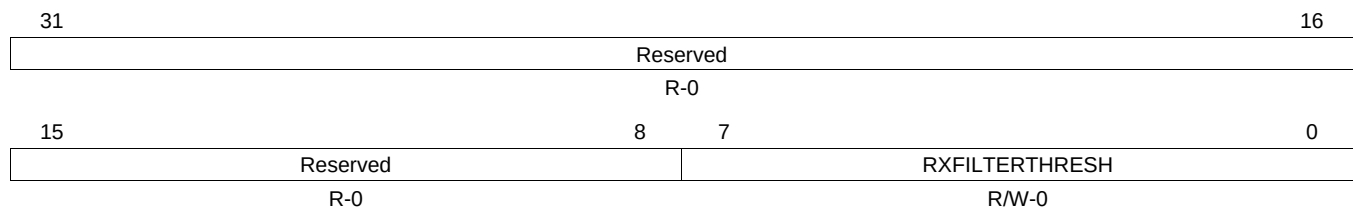
Figure 29-67. Receive Filter Low Priority Frame Threshold Register (RXFILTERLOWTHRESH)
