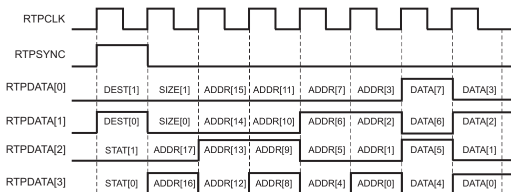
Figure 31-8. Packet Format in Trace Mode
