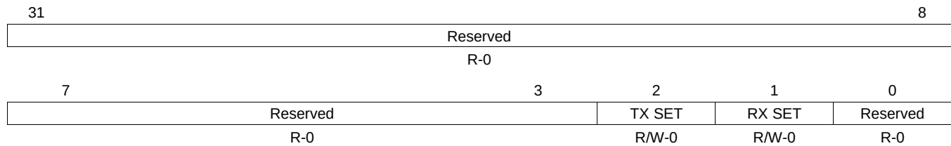
Figure 25-46. SCI Pin I/O Control Register 4 (SCIPIO4) [offset = 4Ch]
