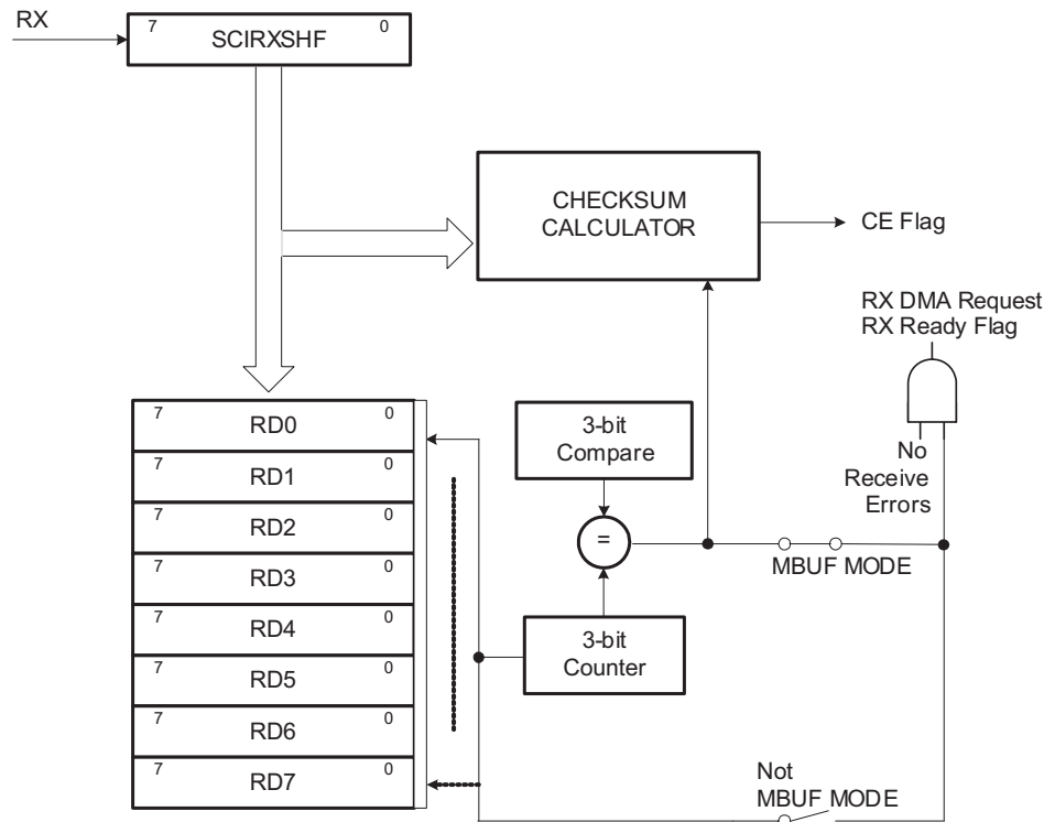
Figure 25-8. Receive Buffers
