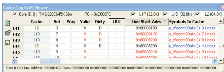
Figure 5-22. Cache Tag RAM Viewer
