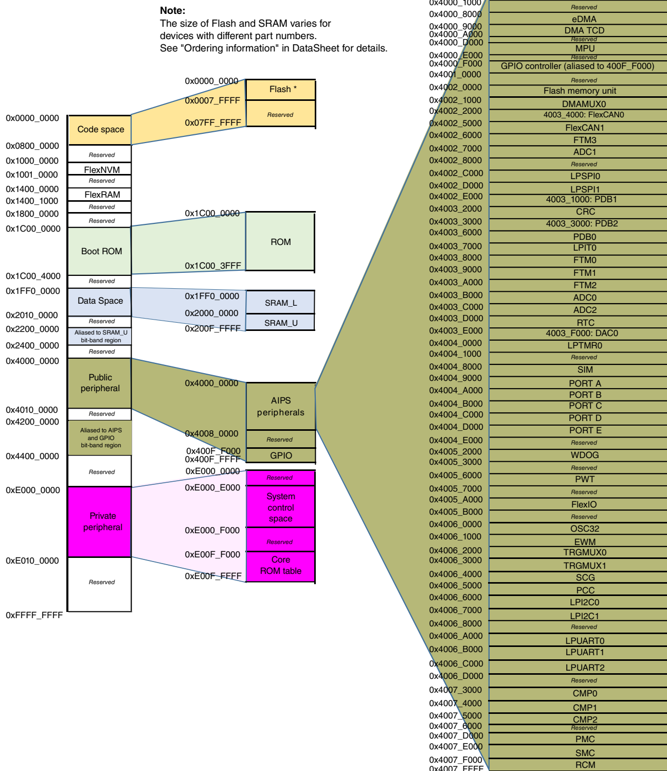
Figure 6. Memory map
