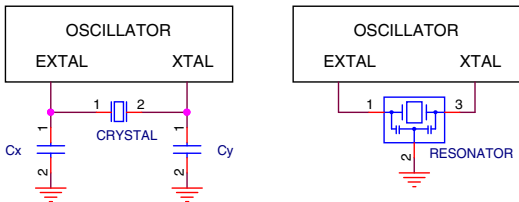
Figure 41. Crystal connection – Diagram 2
