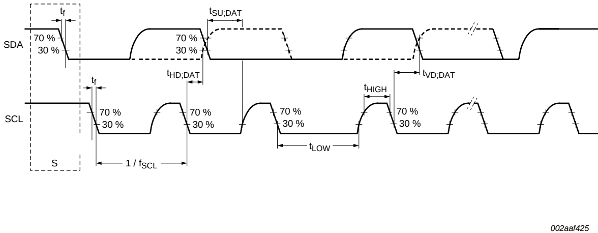
Fig 15. I 2 C-bus pins clock timing
