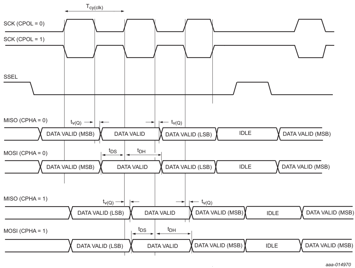
Fig 20. SPI slave timing
