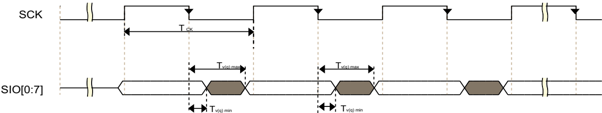
Fig 26. SDR mode (output timing, mode 0 and 1)
