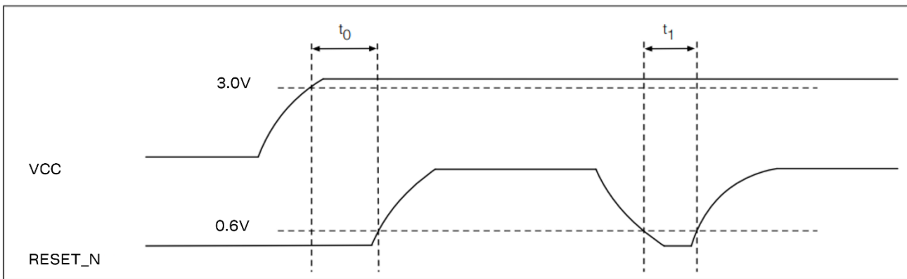
Figure 4: Module power-up and reset timing
