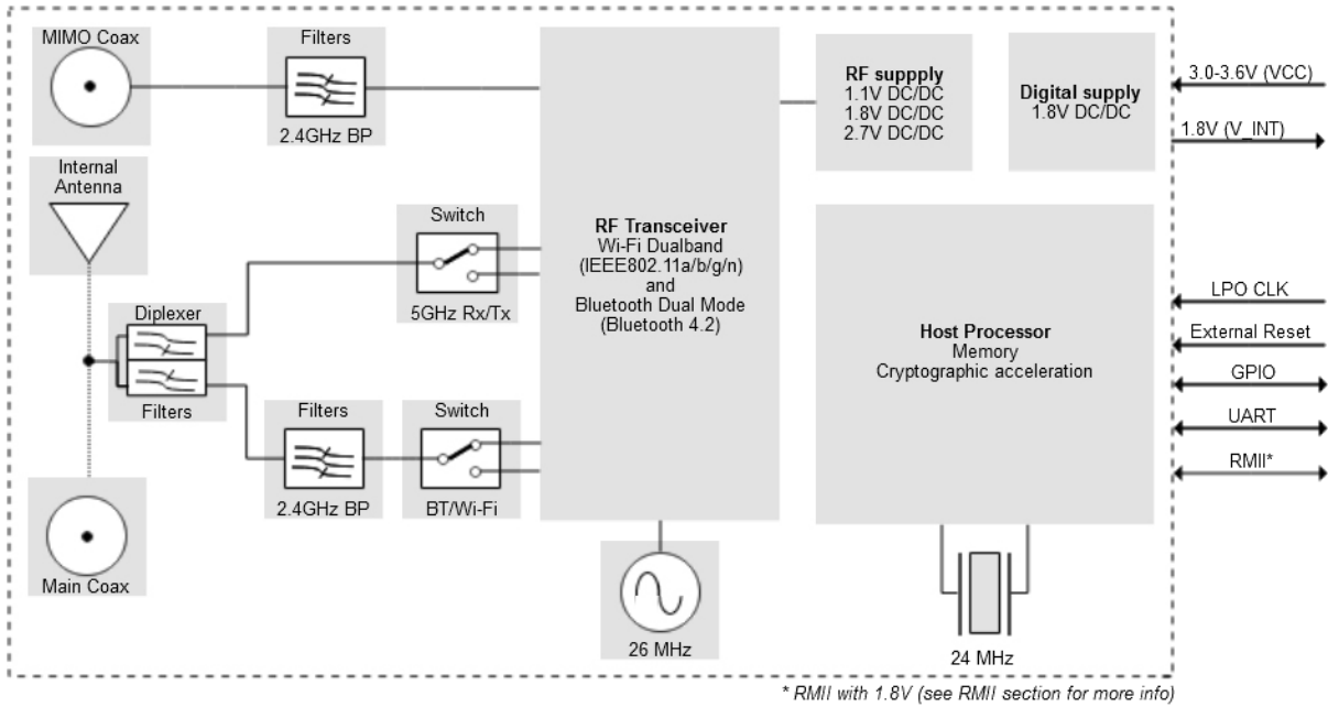
Figure 1: ODIN-W2 series block diagram
