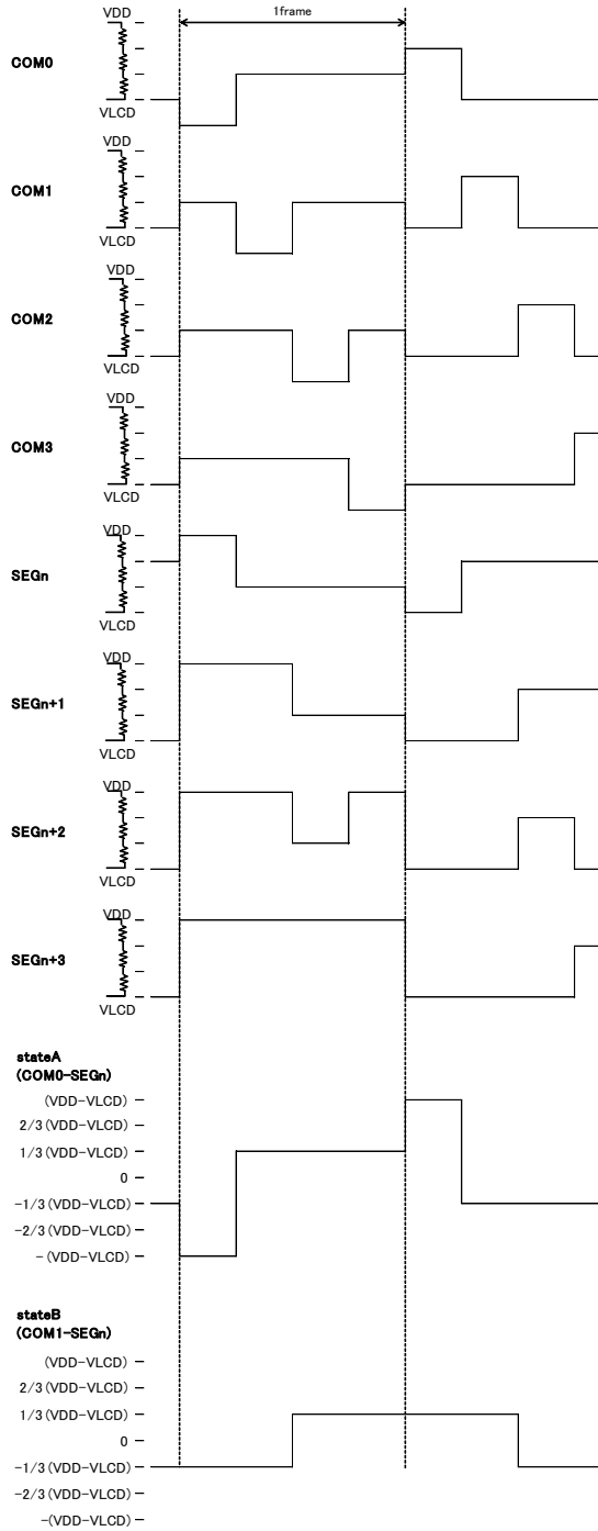
Figure 16. LCD Waveform at Frame Inversion (1/3bias)
