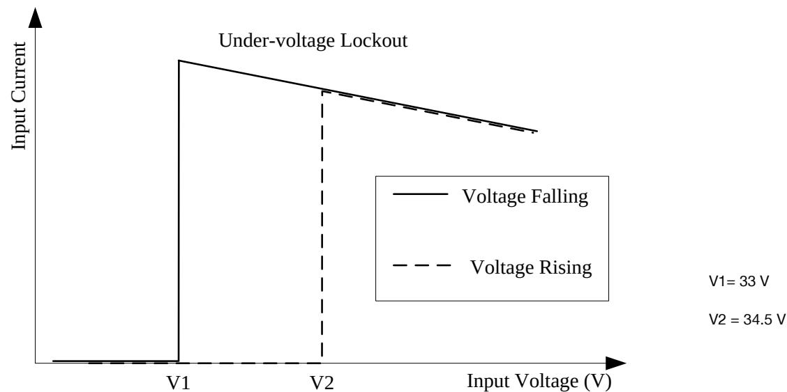
Figure 18. Input under-voltage lockout
