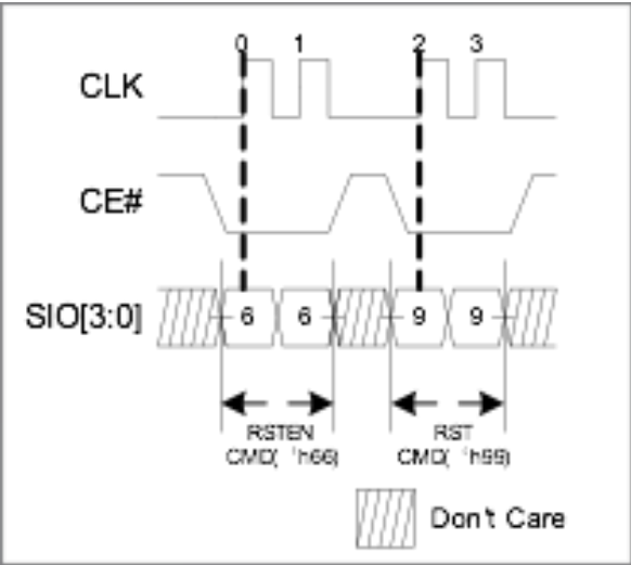
Figure 8-2. QPI Reset
