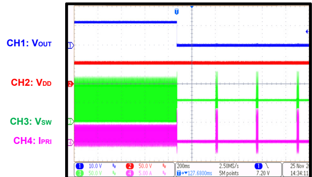
SCP Entry I_{OUT} = 6A to short
