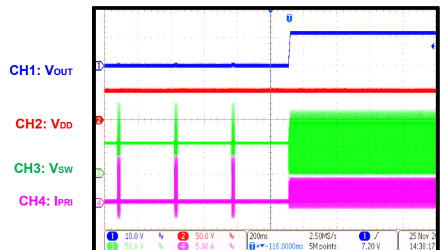
SCP Recovery I_{OUT} = \text{short to } 6A
