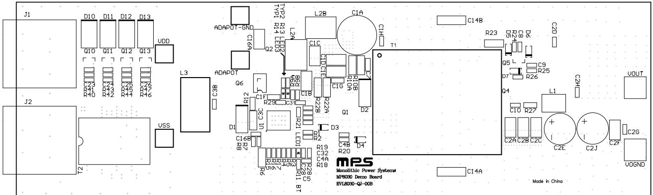
Figure 2: Top Silk
