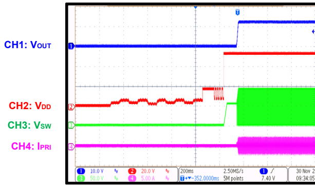
Start-Up through PSE
