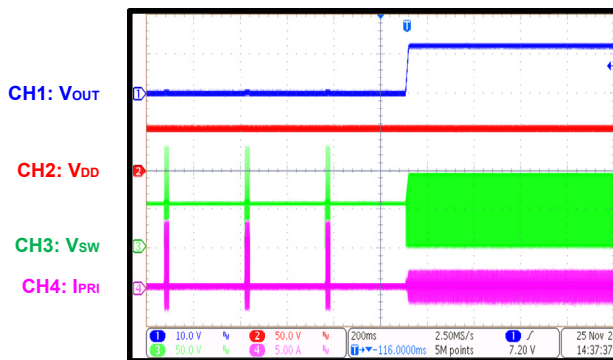
SCP Recovery I_{OUT} = \text{short to } 0A
