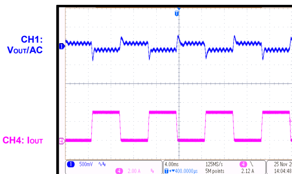
Load Transient I_{OUT} = 0A to 3A , I_{RAMP} = 25mA/\mu s
