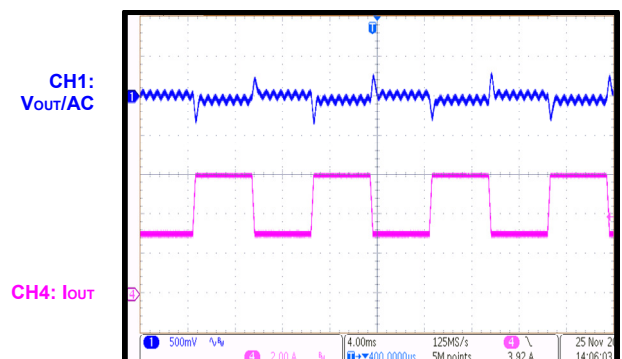
Load Transient I_{OUT} = 3A to 6A , I_{RAMP} = 25mA/\mu s
