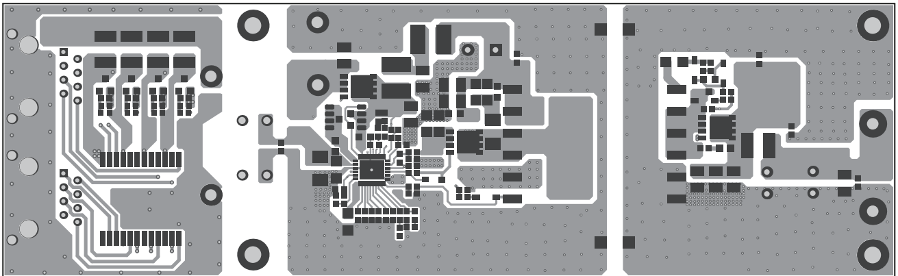
Figure 3: Top Layer
