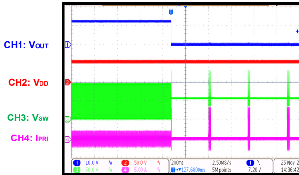
SCP Entry I_{OUT} = 0A to short
