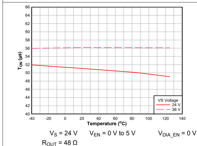
Figure 7-5. Turn-on Time (t ON ) vs Temperature
