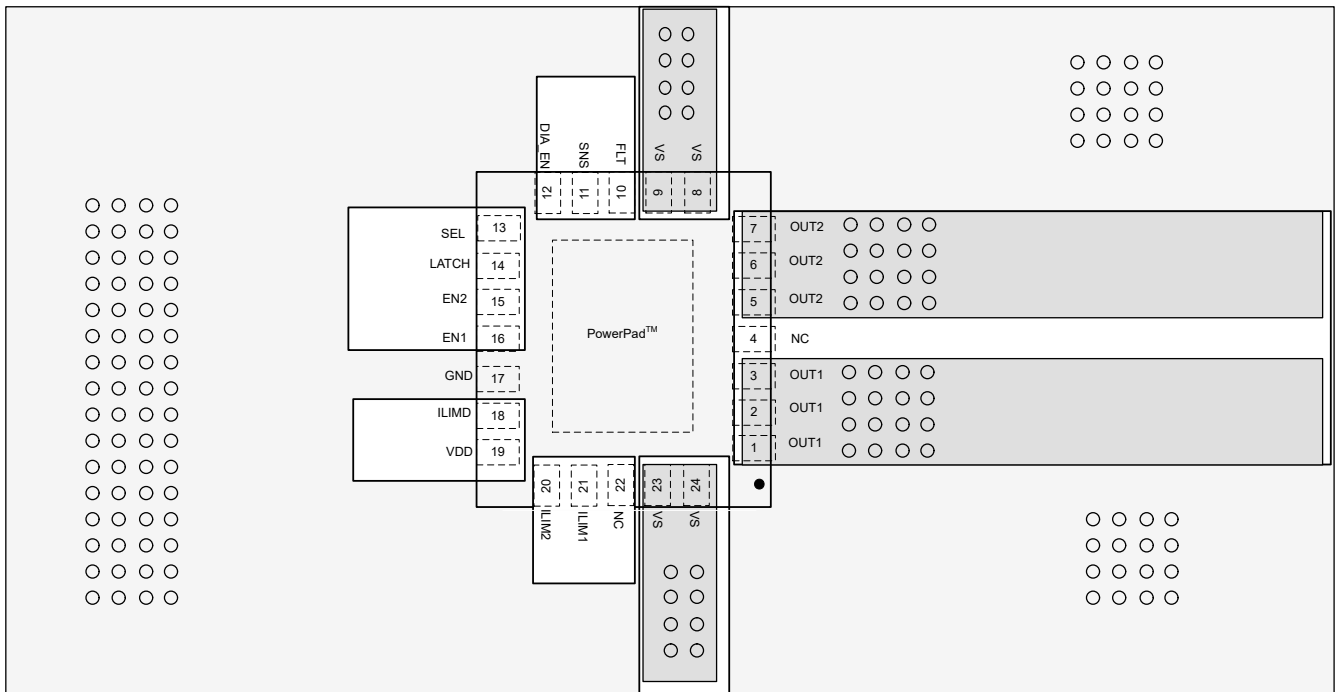
Figure 10-10. Layout Example
