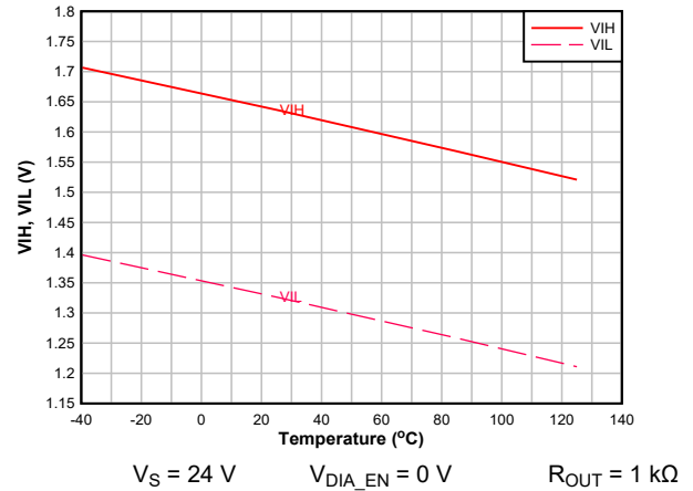
Figure 7-8. V_{IH} , V_{IL} vs Temperature
