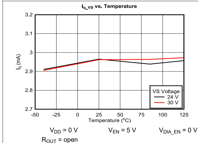
Figure 7-3. Quiescent Current (I Q_VS_SS ) From VS Input Supply vs Temperature
