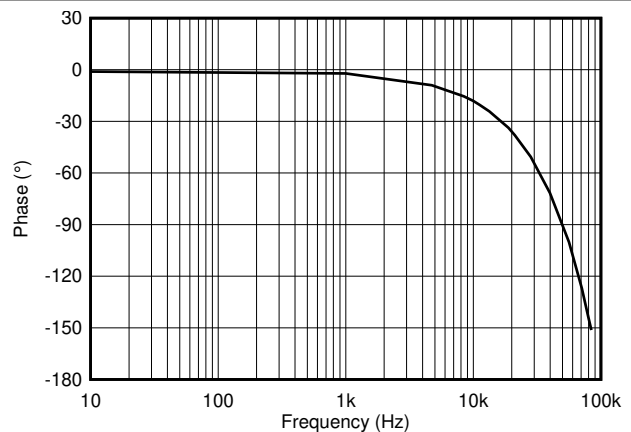
Figure 7-18. Phase vs. Frequency, All Gains
