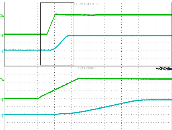
Figure 13: Input Voltage Start-up at open load Time: 10ms/div. Vin (top trace): 20V/div; Vout (bottom trace): 10V/div.
