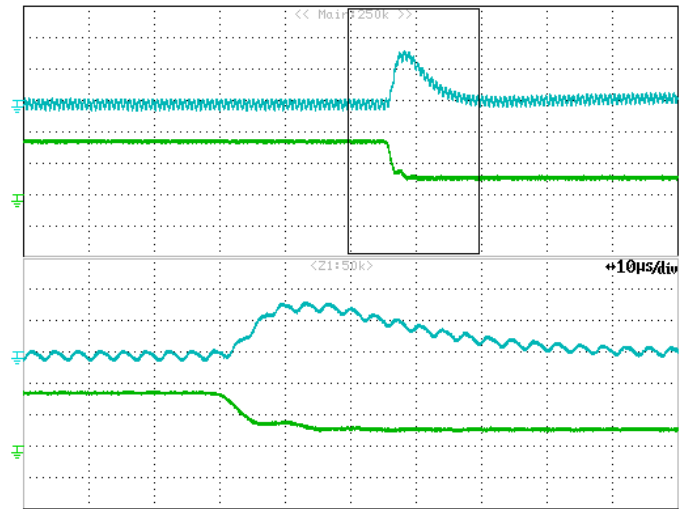
Figure 16: Transient Response
