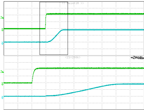
Figure 11: Remote On/Off Start-up at open load Time: 10ms/div. Vremote On/Off signal(top trace): 2V/div; Vout (bottom trace): 10V/div.
