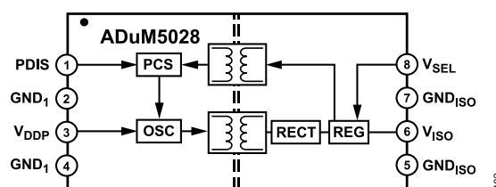
Figure 2. ADuM5028 Functional Block Diagram
