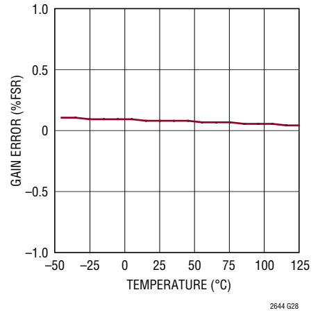
Gain Error vs Temperature
