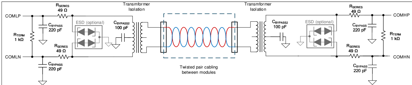
Figure 10-10. Transformer Isolation
