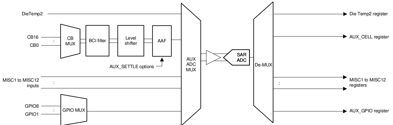
Figure 8-7. AUX ADC Measurement Path
