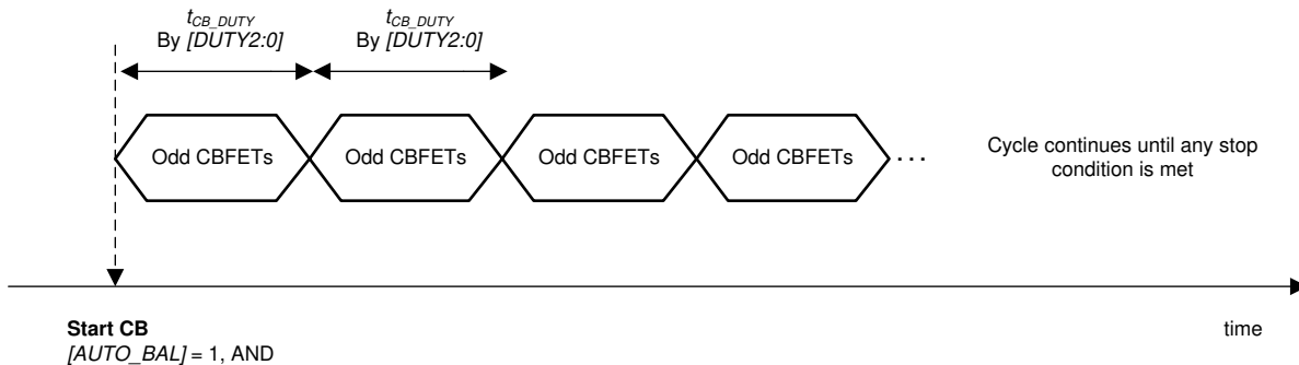
Figure 8-16. Auto Balancing Control, Example 2
