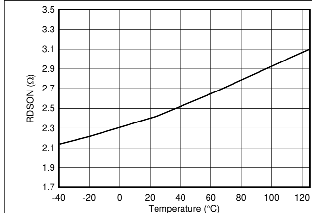
Figure 7-3. CBFET RDSON vs Temperature
