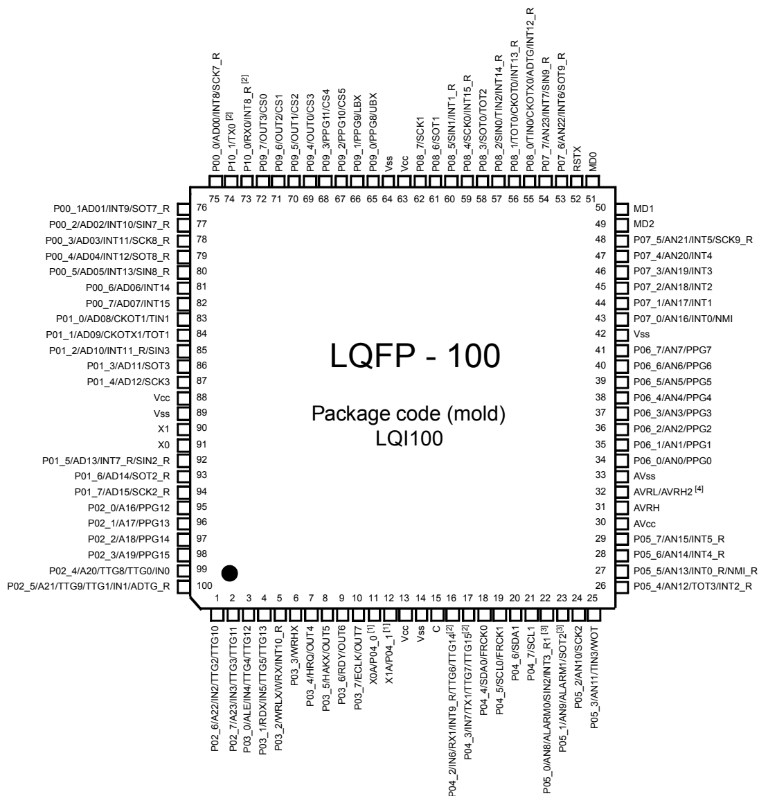
Figure 3. Pin assignment of CY96(F)34x (LQ100)
