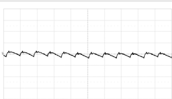
Fundamental output voltage ripple at V_i = 12\text{ V} , I_o = 50\text{ A} , C_{OUT} = 4 \times 330\text{ }\mu\text{F}/10\text{ m}\Omega + 12 \times 100\text{ }\mu\text{F} Scale: 5 mV/div, 1 \mu\text{s}/\text{div} , 20 MHz bandwidth. See section Output Ripple and Noise.
