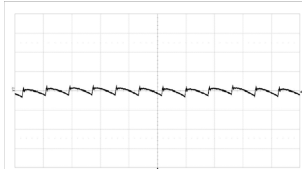
Fundamental output voltage ripple at V_i = 12 V , I_o = 25 A , C_{OUT} = 2 \times 330 \mu\text{F}/10 \text{ m}\Omega + 6 \times 100 \mu\text{F} Scale: 10 mV/div, 2 \mu\text{s}/\text{div} , 20 MHz bandwidth. See section Output Ripple and Noise.
