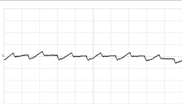
Fundamental output voltage ripple at V_i = 12\text{ V} , I_o = 20\text{ A} , C_{OUT} = 4 \times 330\text{ }\mu\text{F}/10\text{ m}\Omega + 12 \times 100\text{ }\mu\text{F} Scale: 5 mV/div, 1 \mu\text{s} /div, 20 MHz bandwidth. See section Output Ripple and Noise.
