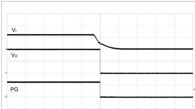
Output disabled by removing V_i . V_i = 12\text{ V} , I_o = 25\text{ A} . Scale from top: 10, 0.5, 2 V/div, 20 ms/div.
