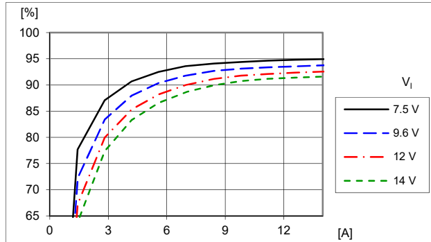
Efficiency vs. load current and input voltage.
