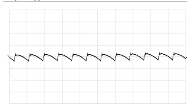
Fundamental output voltage ripple at V_i = 12\text{ V} , I_o = 25\text{ A} , C_{OUT} = 2 \times 330\text{ }\mu\text{F}/10\text{ m}\Omega + 6 \times 100\text{ }\mu\text{F} Scale: 10 mV/div, 2 \mu\text{s} /div, 20 MHz bandwidth. See section Output Ripple and Noise.
