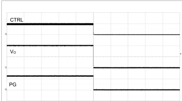
Output disabled by CTRL pin. V_i = 12\text{ V} , I_o = 25\text{ A} . Scale from top: 5, 0.5, 2 V/div, 20 ms/div.
