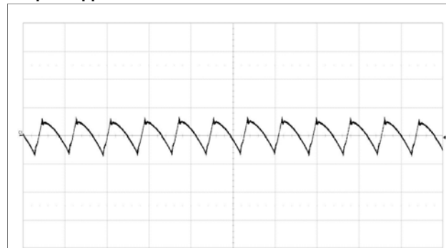
Fundamental output voltage ripple at V_i = 12\text{ V} , I_o = 17\text{ A} , C_{OUT} = 2 \times 330\text{ }\mu\text{F}/10\text{ m}\Omega + 6 \times 100\text{ }\mu\text{F} Scale: 10 mV/div, 2 \mu\text{s}/\text{div} , 20 MHz bandwidth. See section Output Ripple and Noise.
