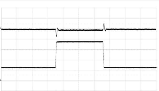
Output voltage response to load current step change (25%–75%–25%) at V_i = 12\text{ V} , C_{OUT} = 4 \times 330\text{ }\mu\text{F}/10\text{ m}\Omega + 12 \times 100\text{ }\mu\text{F} , di/dt = 2\text{ A}/\mu\text{s} , ACSR Gain=200 and ACSR Residual=90. Scale from top: 50 mV/div, 10 A/div, 200 \mu\text{s}/\text{div} . Note: Sense pins are connected to load.
