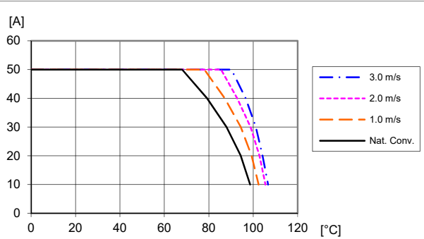
Available load current vs. ambient air temperature and airflow at V_i = 12\text{ V} .
