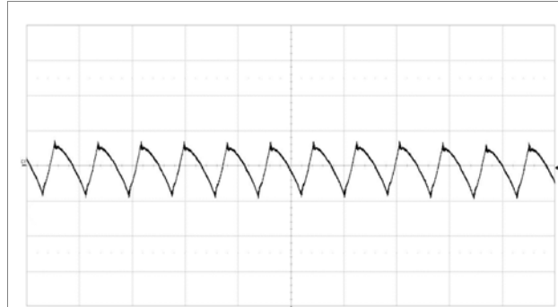
Fundamental output voltage ripple at V_i = 12\text{ V} , I_o = 14\text{ A} , C_{OUT} = 2 \times 330\text{ }\mu\text{F}/10\text{ m}\Omega + 6 \times 100\text{ }\mu\text{F} Scale: 10 mV/div, 2 \mu\text{s}/\text{div} , 20 MHz bandwidth. See section Output Ripple and Noise.
