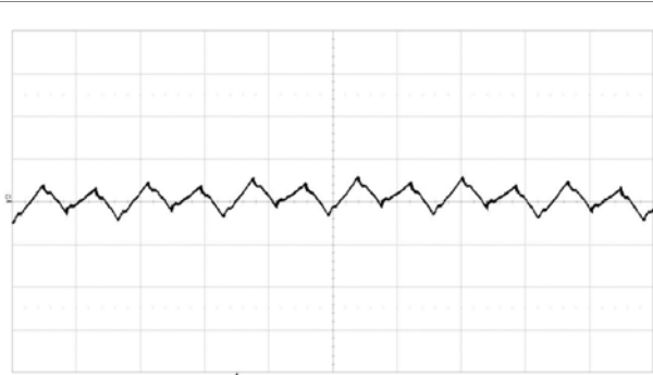
Fundamental output voltage ripple at V_i = 12\text{ V} , I_o = 28\text{ A} , C_{OUT} = 4 \times 330\text{ }\mu\text{F}/10\text{ m}\Omega + 12 \times 100\text{ }\mu\text{F} Scale: 5 mV/div, 1 \mu\text{s} /div, 20 MHz bandwidth. See section Output Ripple and Noise.
