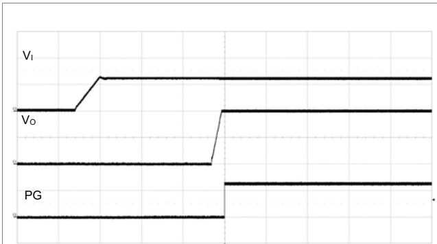
Output enabled by applying V_i . V_i = 12\text{ V} , I_o = 25\text{ A} . T_{ON\_DELAY} = T_{ON\_RISE} = 5\text{ ms} , POWER\_GOOD\_DELAY = 1\text{ ms} . USER\_CONFIG = 0x1084 (page0) / 0x10A4 (page1) (default). Scale from top: 10, 0.5, 2 V/div, 20 ms/div.
