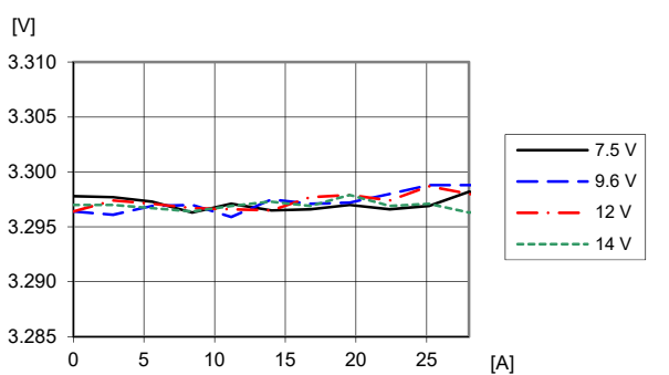
Output voltage vs load current.
