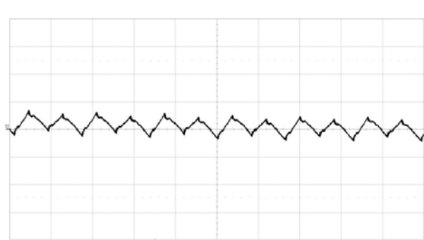
Fundamental output voltage ripple at V_i = 12\text{ V} , I_o = 34\text{ A} , C_{OUT} = 4 \times 330\text{ }\mu\text{F}/10\text{ m}\Omega + 12 \times 100\text{ }\mu\text{F} Scale: 5 mV/div, 1 \mu\text{s} /div, 20 MHz bandwidth. See section Output Ripple and Noise.
