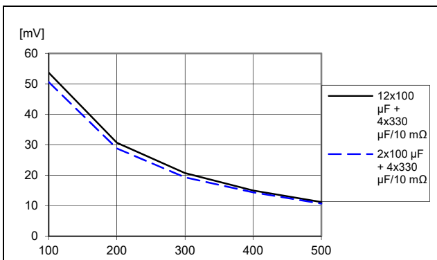
Load transient peak voltage deviation vs. ASCR gain and external capacitance. Step (12.5–37.5–12.5 A). V_i = 12\text{ V} , V_o = 1.0\text{ V} , f_{sw} = 615\text{ kHz} , ASCR residual = 90, di/dt = 2\text{ A}/\mu\text{s} . ASCR gain changed by PMBus command ASCR_CONFIG.
