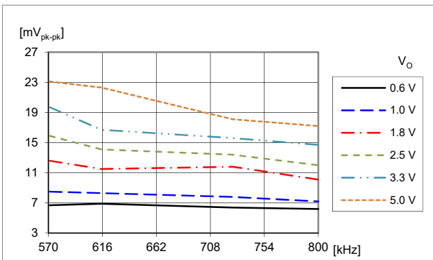
Output voltage ripple V_{pk-pk} vs. switching frequency at V_I = 12\text{ V} , I_O = \text{max } I_O , C_O = 2 \times 330\text{ }\mu\text{F}/10\text{ m}\Omega + 6 \times 100\text{ }\mu\text{F} . Frequency changed by PMBus command FREQUENCY_SWITCH.
