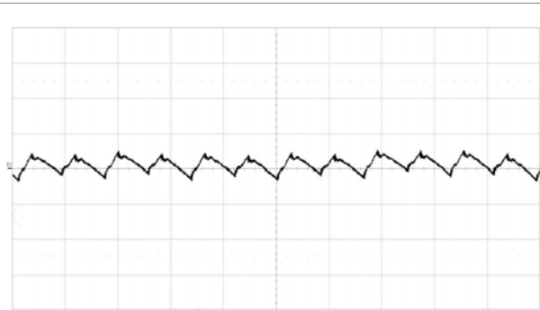
Fundamental output voltage ripple at V_i = 12\text{ V} , I_o = 45\text{ A} , C_{OUT} = 4 \times 330\text{ }\mu\text{F}/10\text{ m}\Omega + 12 \times 100\text{ }\mu\text{F} Scale: 5 mV/div, 1 \mu\text{s} /div, 20 MHz bandwidth. See section Output Ripple and Noise.
