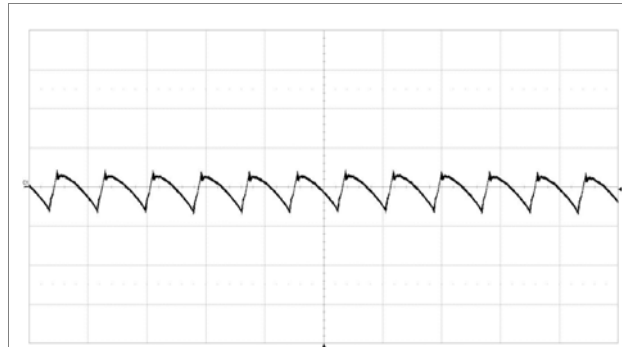
Fundamental output voltage ripple at V_i = 12\text{ V} , I_o = 22.5\text{ A} , C_{OUT} = 2 \times 330\text{ }\mu\text{F}/10\text{ m}\Omega + 6 \times 100\text{ }\mu\text{F} Scale: 10 mV/div, 2 \mu\text{s}/\text{div} , 20 MHz bandwidth. See section Output Ripple and Noise.
