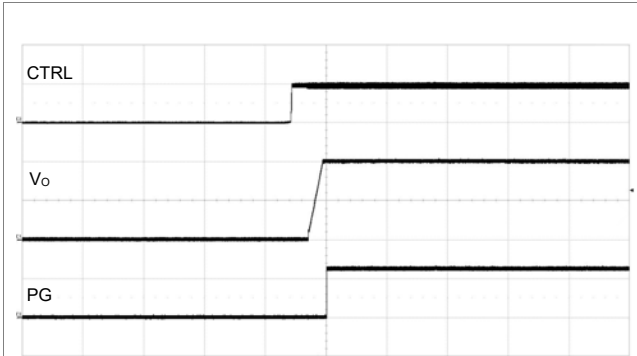
Output enabled by CTRL pin. V_i = 12\text{ V} , I_o = 25\text{ A} . T_{ON\_DELAY} = T_{ON\_RISE} = 5\text{ ms} , POWER\_GOOD\_DELAY = 1\text{ ms} . Scale from top: 5, 0.5, 2 V/div, 20 ms/div.
