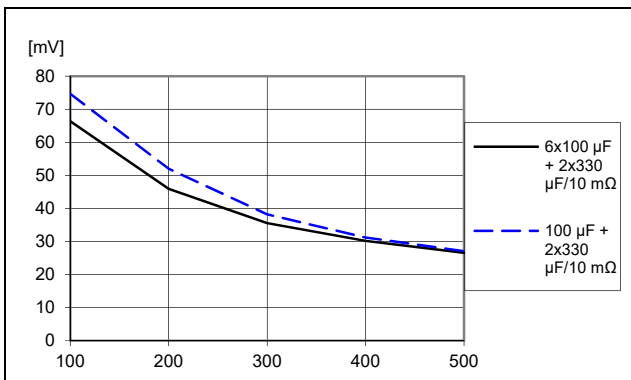
Load transient peak voltage deviation vs. ASCR gain and external capacitance. Step (6.25–18.75–6.25 A). V_I = 12\text{ V} , V_O = 1.0\text{ V} , f_{sw} = 615\text{ kHz} , ASCR residual = 90, di/dt = 2\text{ A}/\mu\text{s} . ASCR gain changed by PMBus command ASCR_CONFIG.
