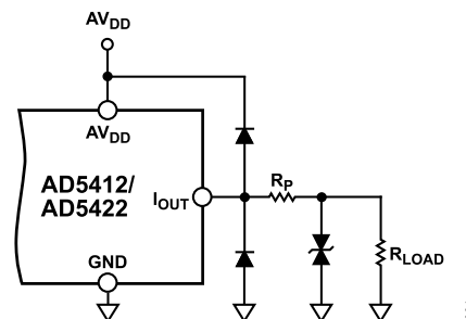
Figure 78. Output Transient Voltage Protection
