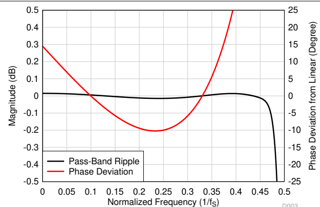
Figure 7-56. Ultra-Low-Latency Decimation Filter Pass-Band Ripple and Phase Deviation
