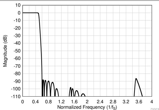
Figure 7-55. Ultra-Low-Latency Decimation Filter Magnitude Response
