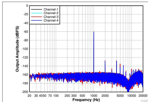
Figure 8-2. FFT With a -60-dBr Input
