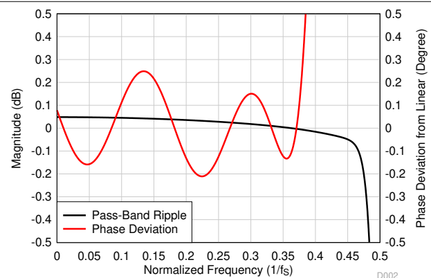
Figure 7-38. Low-Latency Decimation Filter Pass-Band Ripple and Phase Deviation
