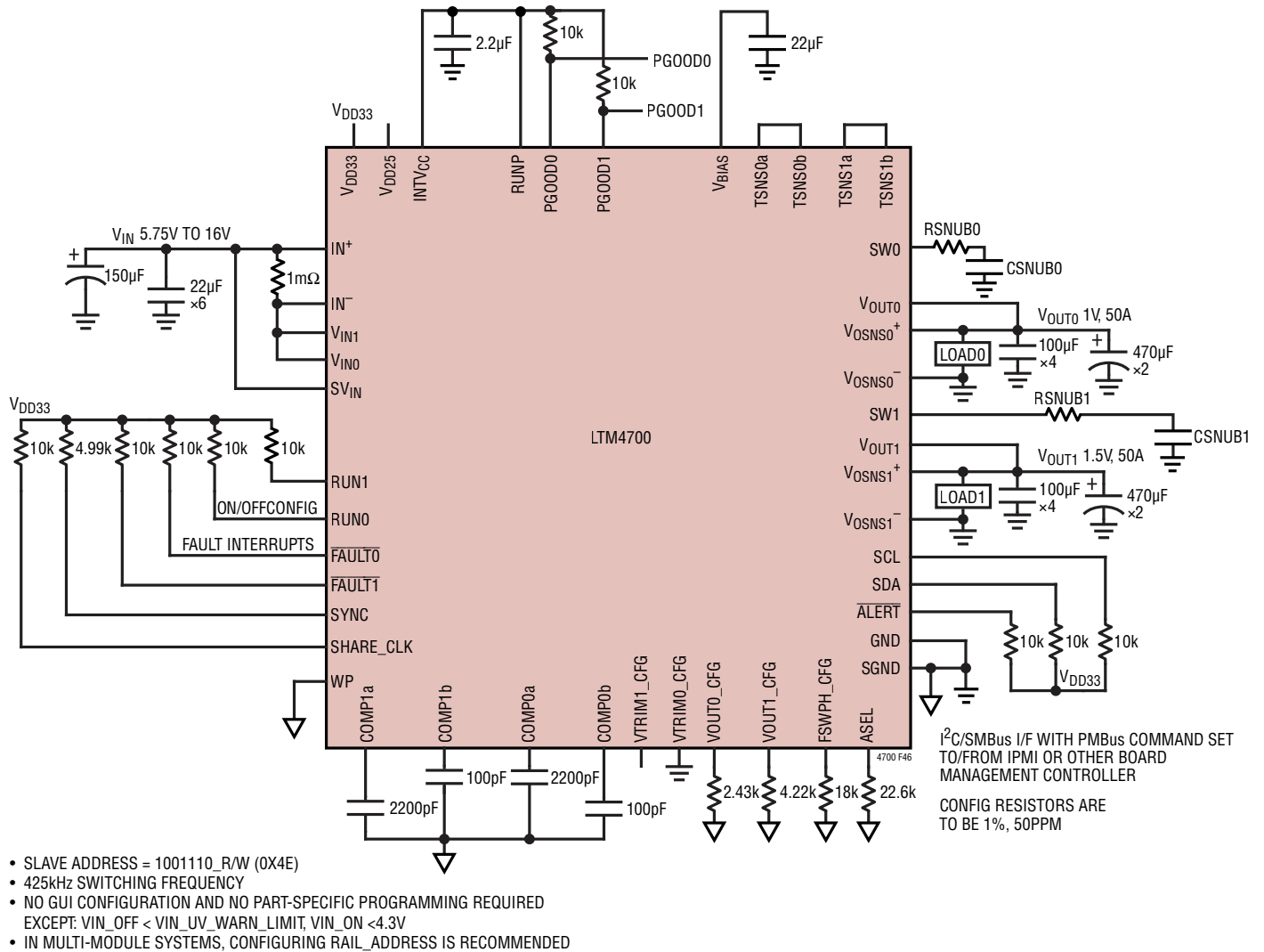
Figure 46. 1.0V and 1.5V Outputs at 50A With Providing I 2 C/SMBus/PMBus Serial Interface
