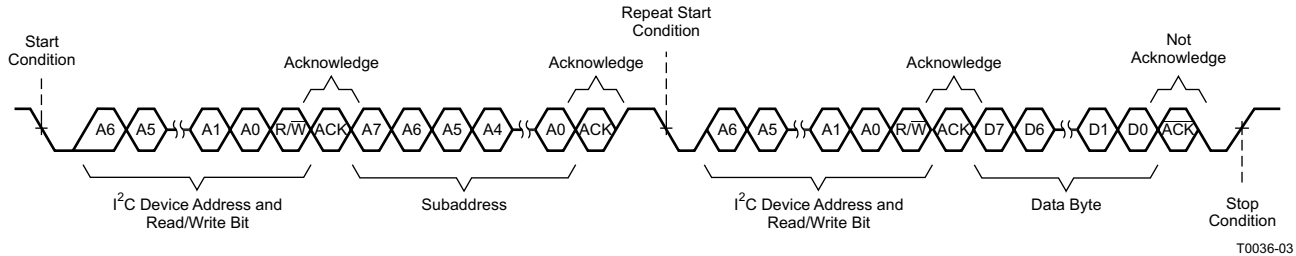
Figure 7-6. Random Read Transfer
