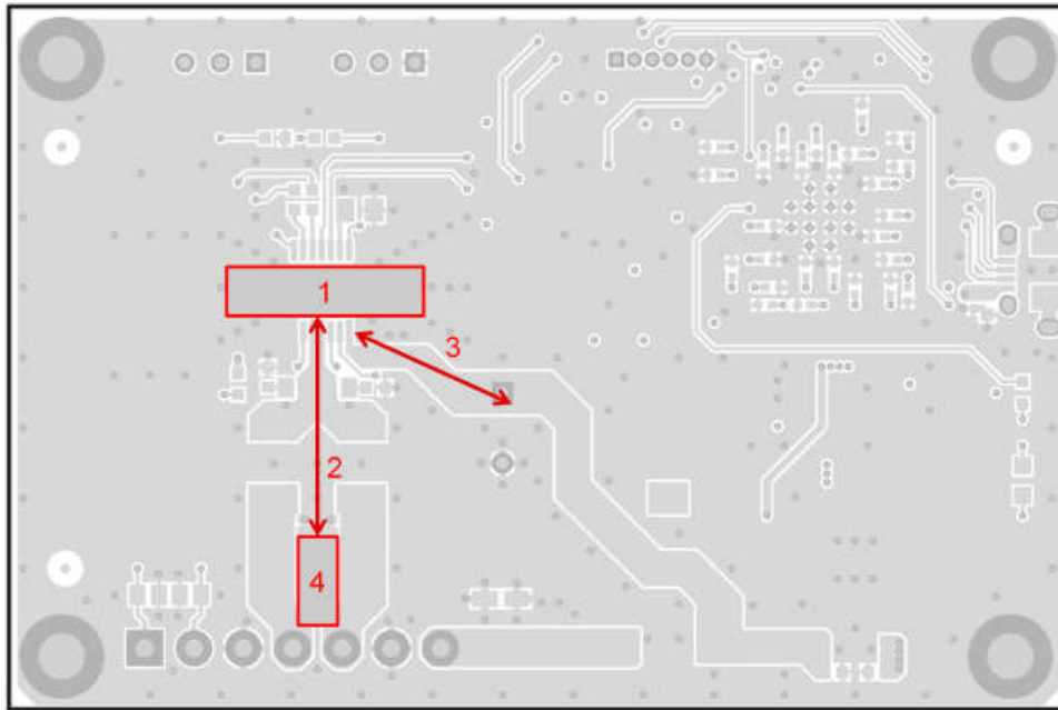
Figure 9-1. Top layer
