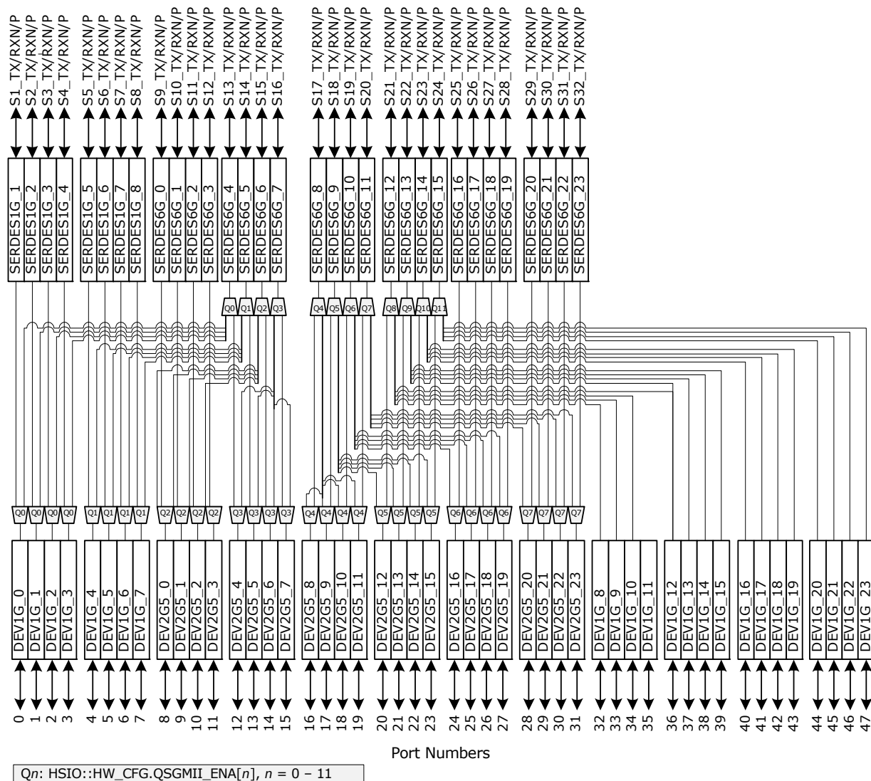
Figure 16 • QSGMII Muxing
