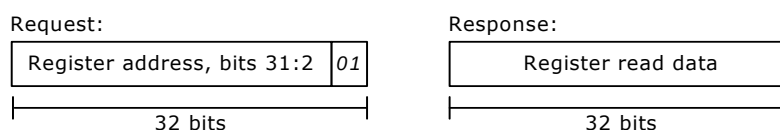
Figure 118 • READ Command
