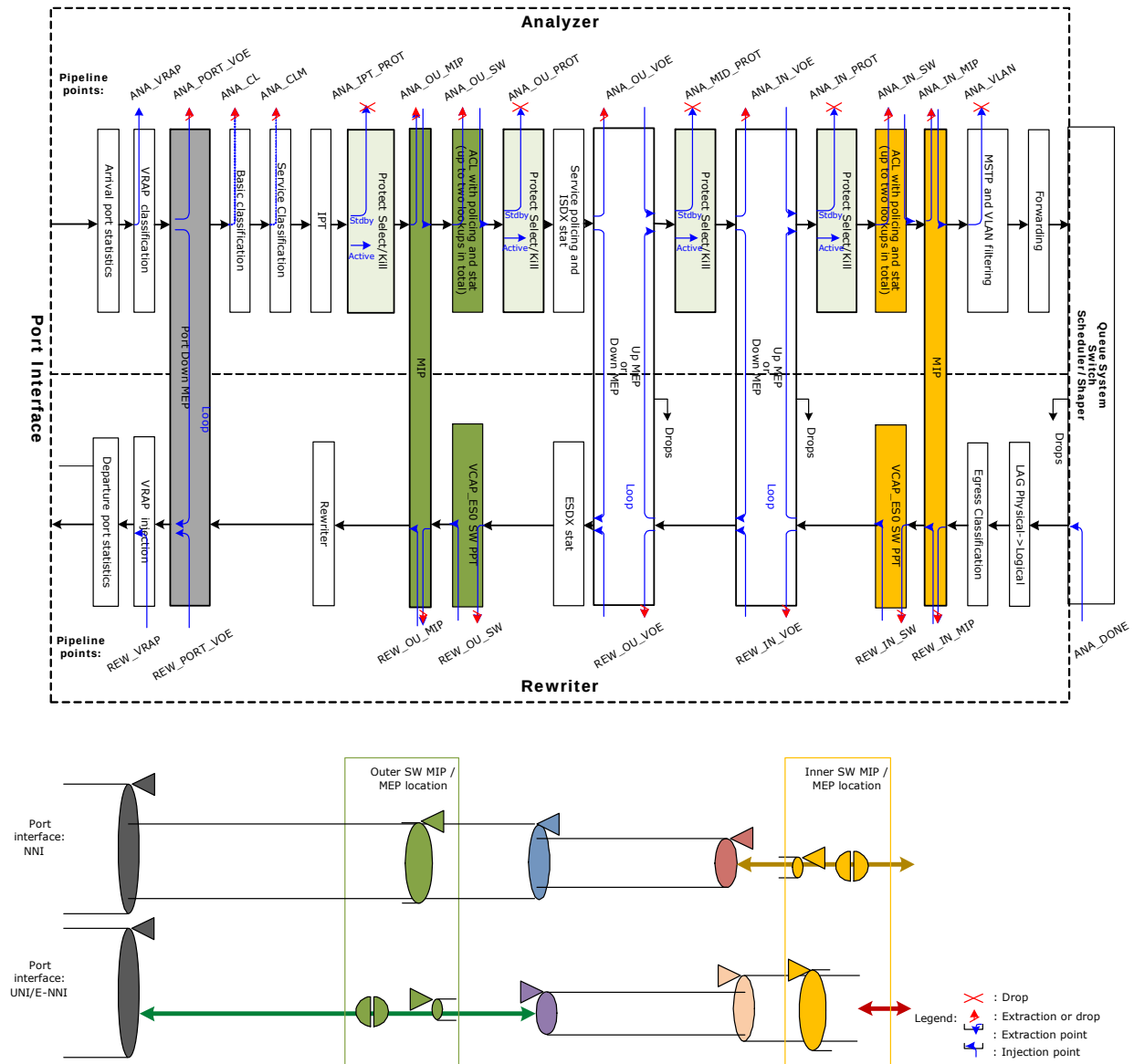
Figure 21 • Processing Flow
