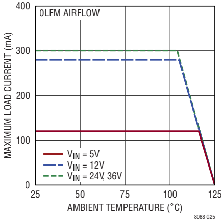
Derating, 1.8 V_{OUT2}
