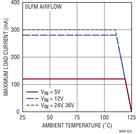
Derating, 1.2 V_{OUT2}
