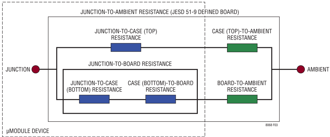
Figure 3. Approximate Thermal Model of LTM8068
