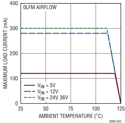
Derating, 2.5 V_{OUT2}
