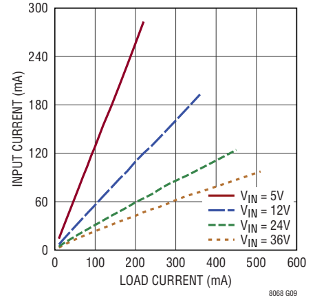
Input Current vs Load Current, V_{OUT1} = 5\text{V}
