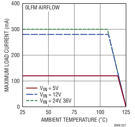
Derating, 3.3 V_{OUT2}
