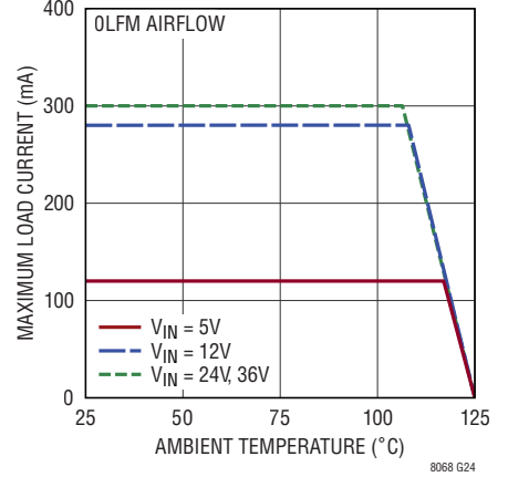
Derating, 1.5 V_{OUT2}
