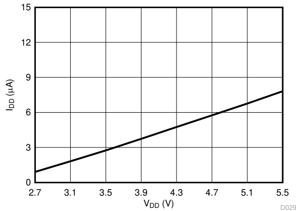
Figure 7-29. Supply Current vs Supply Voltage
