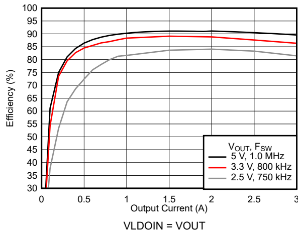
Figure 6-13. Efficiency
