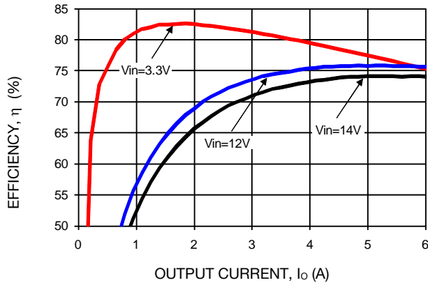
Figure 1. V_o = 0.6 V
