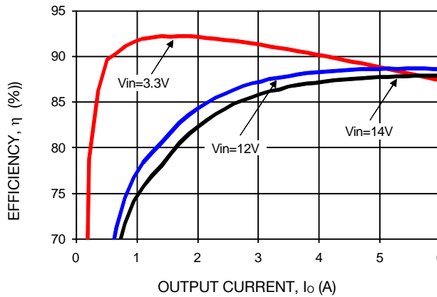
Figure 3. V_o = 1.8 V
