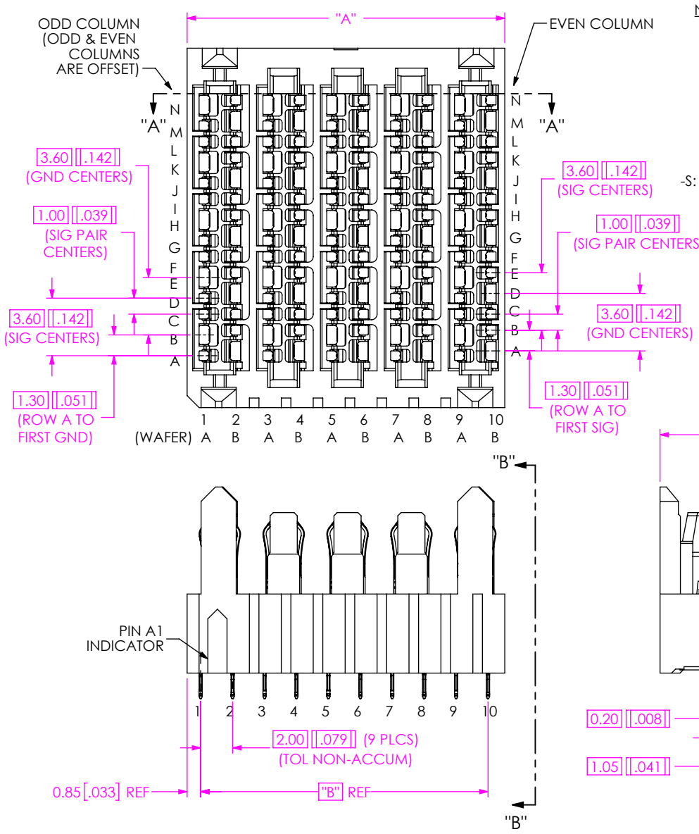
FIG 1 EBTM-4-10-2.0-X-VT-1 SHOWN
