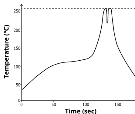
WAVE SOLDERING PROFILE
