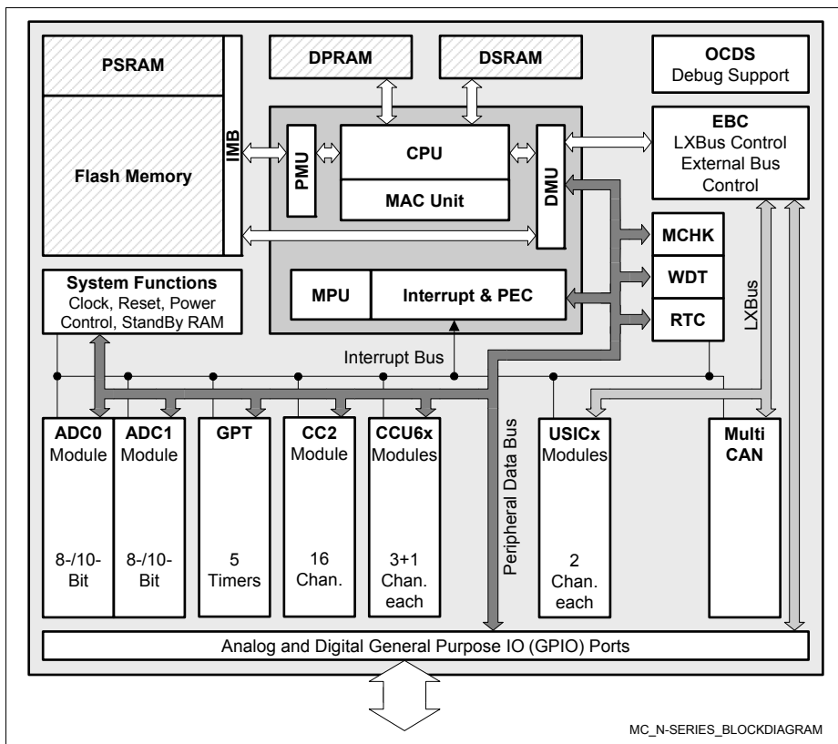
Figure 4 Block Diagram
