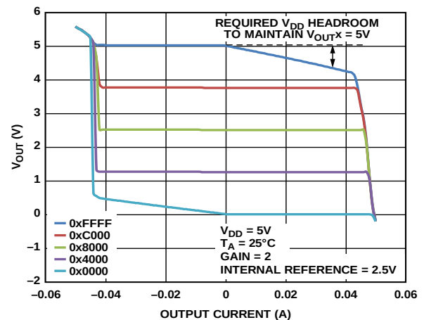
Figure 34. Source and Sink Capability at V_{DD} = 5\text{ V}
