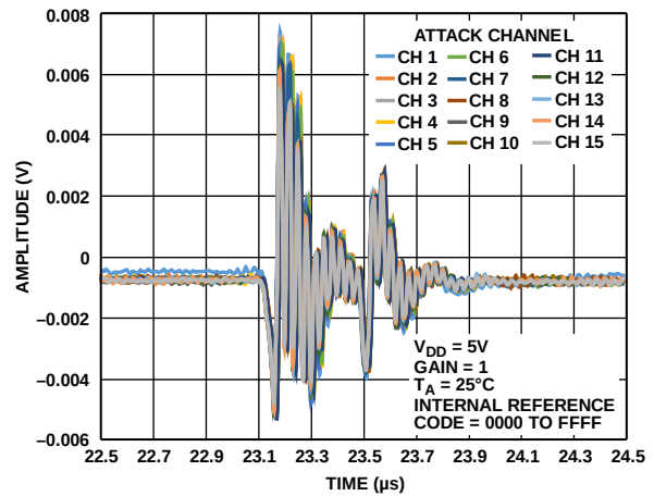
Figure 44. Analog Crosstalk
