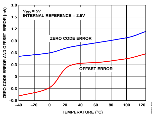
Figure 27. AD5677R Zero Code Error and Offset Error vs. Temperature
