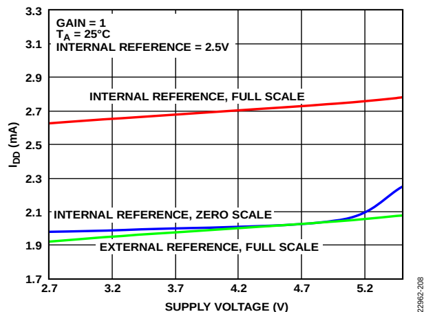
Figure 38. I_{DD} vs. Supply Voltage
