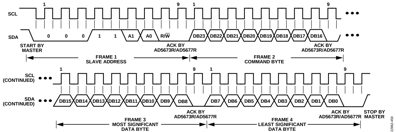
Figure 59. I²C Write Operation
