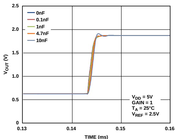
Figure 49. Settling Time at Various Capacitive Loads
