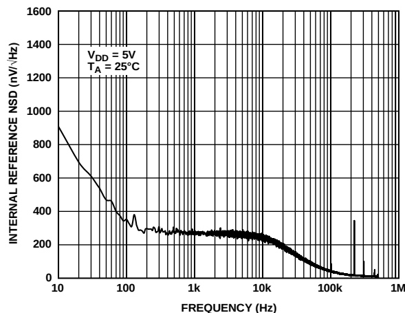
Figure 51. Internal Reference NSD vs. Frequency
