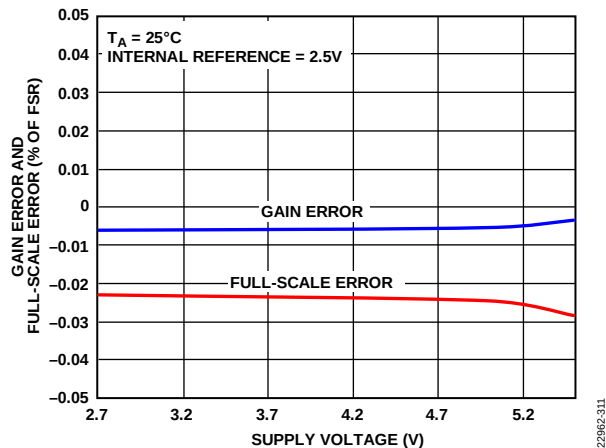
Figure 26. AD5673R Gain Error and Full-Scale Error vs. Supply Voltage
