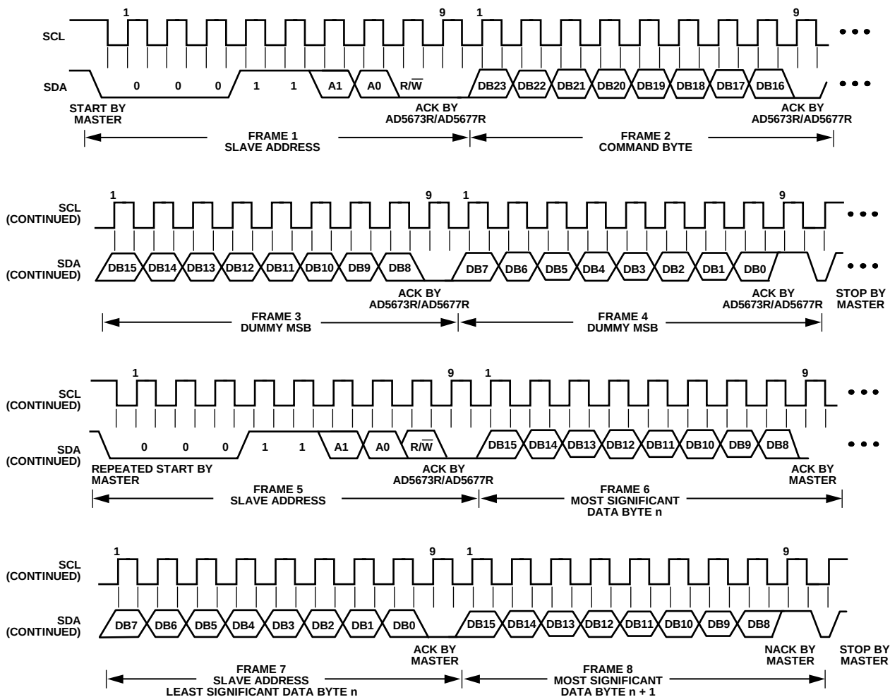
Figure 60. I²C Read Operation
