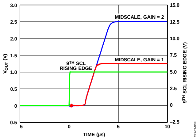
Figure 42. Exiting Power-Down to Midscale
