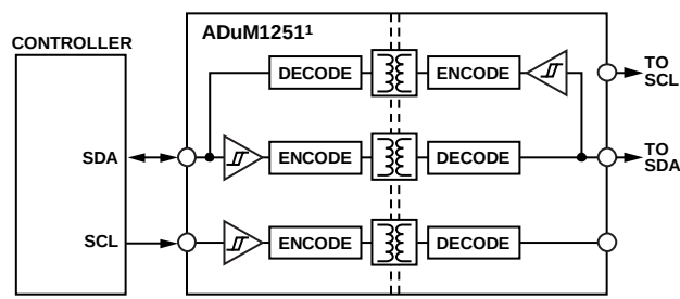
Figure 69. Isolated Interface
