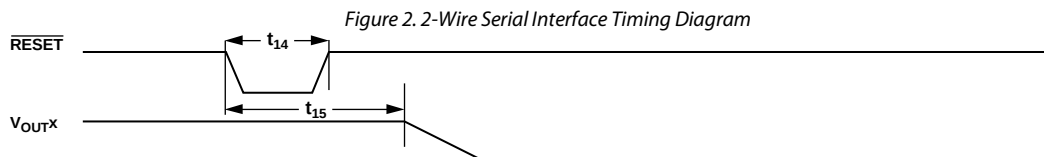
Figure 3. \overline{\text{RESET}} Timing Diagram
