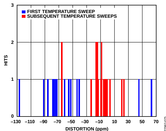
Figure 65. Thermal Hysteresis
