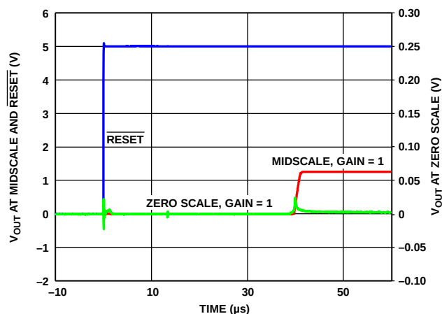
Figure 50. Hardware Reset
