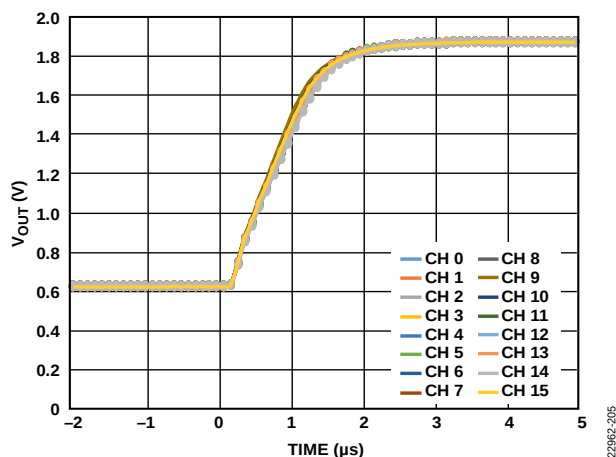
Figure 40. Settling Time
