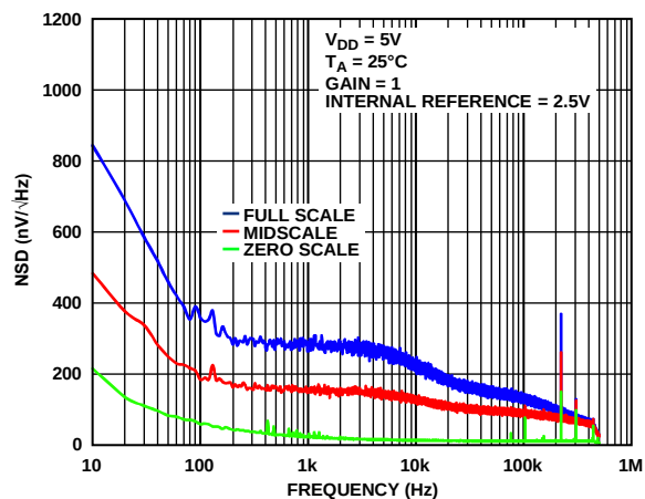
Figure 47. NSD
