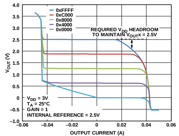
Figure 33. Source and Sink Capability at V_{DD} = 3\text{ V}
