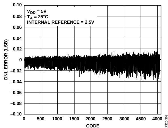
Figure 8. AD5673R DNL Error vs. Code
