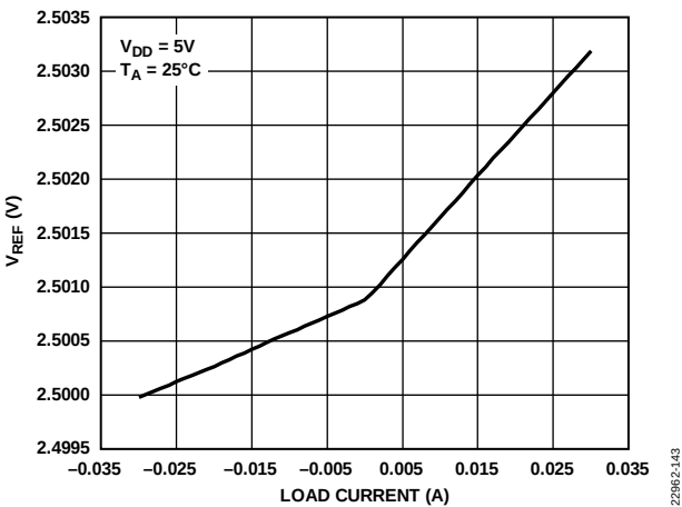
Figure 53. V_{REF} vs. Load Current
