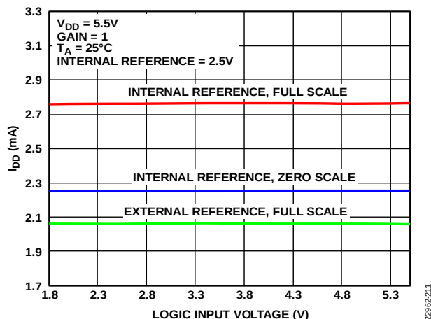
Figure 39. I_{DD} vs. Logic Input Voltage
