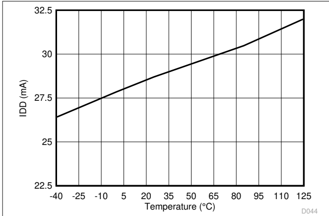
Figure 6-35. Input-Supply Current vs Temperature
