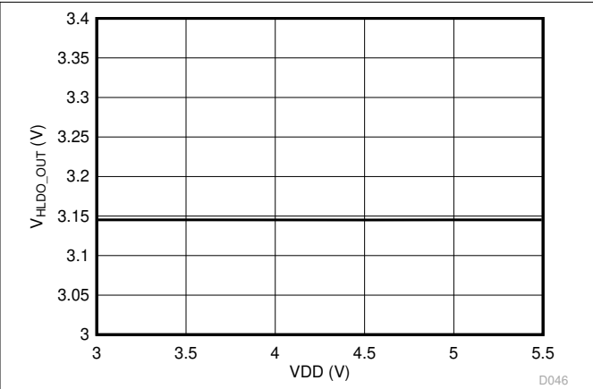
Figure 6-36. High-Side LDO Line Regulation
