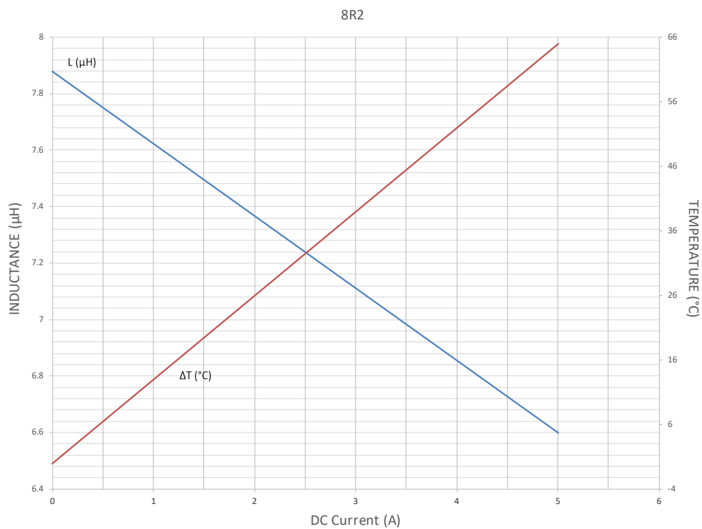
L&I Curve
