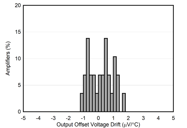
Figure 7-4. Typical Distribution of Output Stage Offset Voltage Drift
