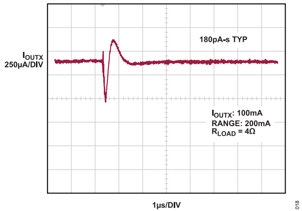
Figure 18. Mid-Scale Glitch
