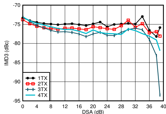
Figure 6-97. TX IMD3 vs DSA Setting at 2.6 GHz
