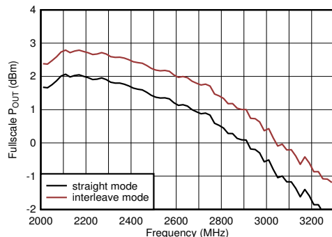
Figure 6-78. TX Full Scale vs RF Frequency at 11796.48MSPS
