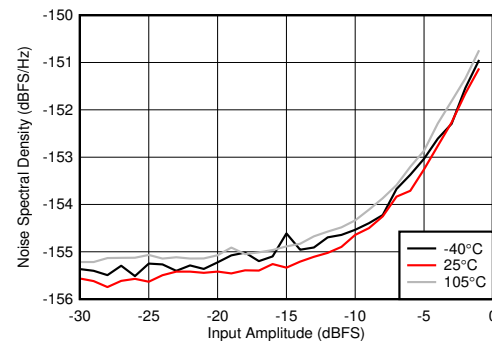
Figure 6-361. RX Noise Spectral Density vs Input Amplitude and Temperature at 2.6 GHz
