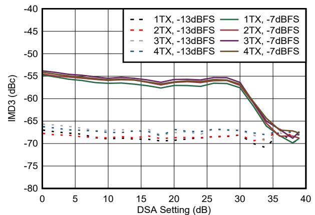
Figure 6-219. TX IMD3 vs DSA Setting at 8.11 GHz
