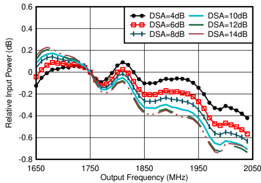
Figure 6-318. RX In-Band Gain Flatness, f_{\text{IN}} = 1750 \text{ MHz}
