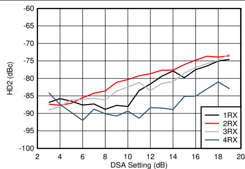
Figure 6-395. RX HD2 vs DSA Setting and Channel at 3.6 GHz
