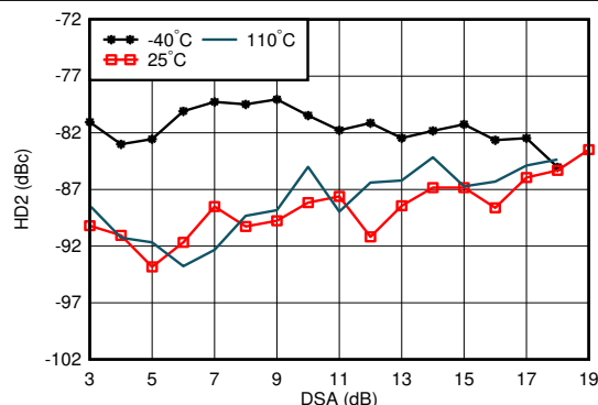
Figure 6-337. RX HD2 vs DSA Setting and Temperature at 1.9 GHz
