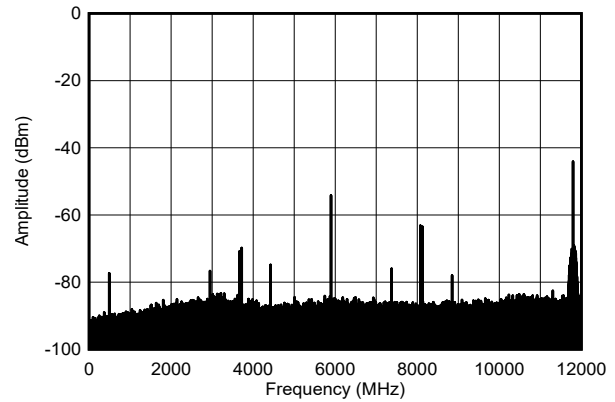
Figure 6-215. TX Dual Tone Output Spectrum at 8.11 GHz
