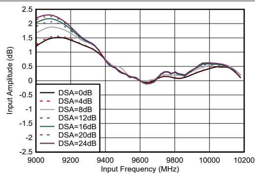
Figure 6-466. RX Input Amplitude vs Frequency at 9.6 GHz
