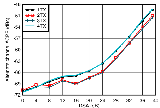
Figure 6-178. TX 20-MHz LTE alt-ACPR vs DSA at 4.9 GHz
