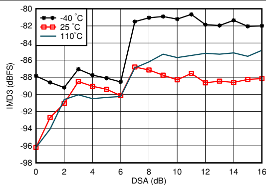
Figure 6-302. RX IMD3 vs DSA Setting and Temperature at 0.8 GHz
