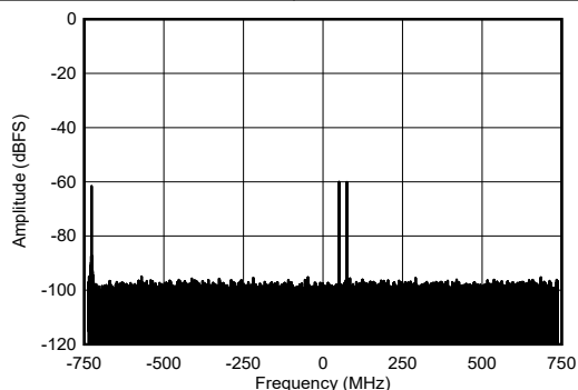
Figure 6-462. RX Dual Tone Output FFT at 8.11GHz
