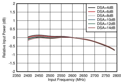
Figure 6-348. RX Inband Gain Flatness, f_{\text{IN}} = 2600 \text{ MHz}
