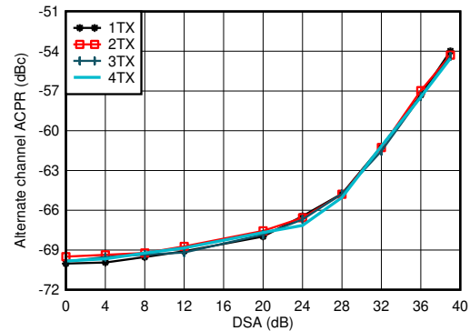
Figure 6-36. TX 20-MHz LTE alt-ACPR vs DSA at 0.85 GHz
