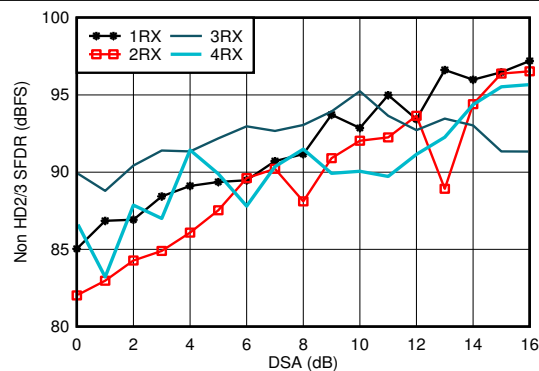
Figure 6-314. RX Non-HD2/3 vs DSA Setting at 0.8 GHz
