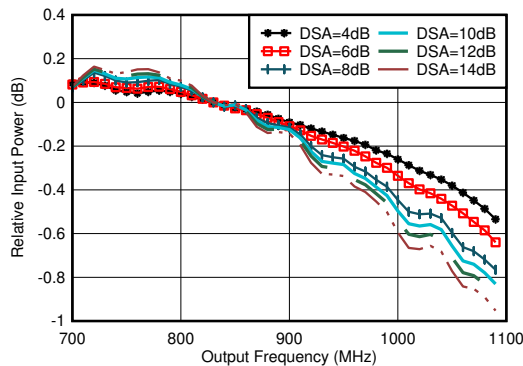
Figure 6-287. RX In-Band Gain Flatness for Channel 1RX, f_{\text{IN}} = 830\text{ MHz}
