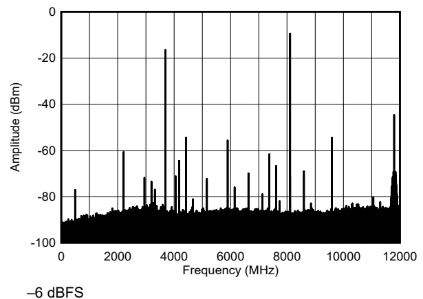
Figure 6-205. TX Single Tone Output Spectrum at 8.11 GHz
