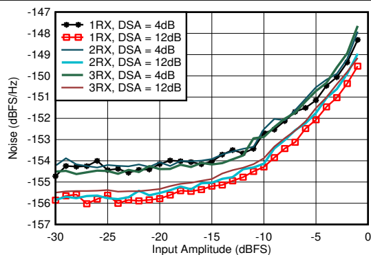
Figure 6-301. RX Noise Spectral Density vs Input Amplitude and Channel at 0.8 GHz
