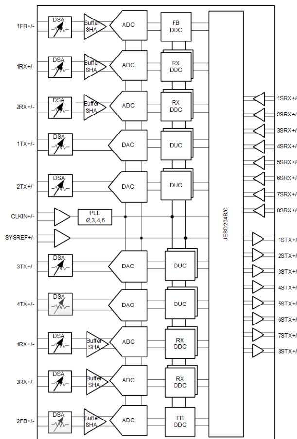
Functional Block Diagram
