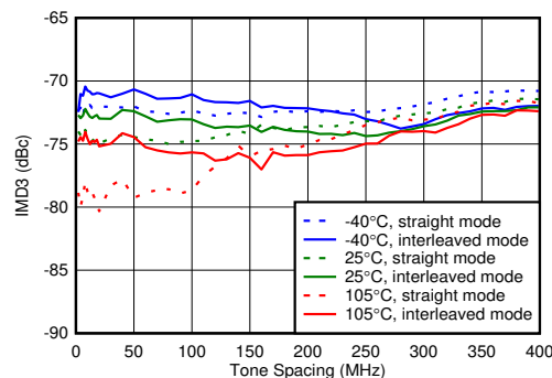
Figure 6-99. TX IMD3 vs Tone Spacing and Temperature at 2.6 GHz
