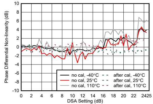
Figure 6-470. RX Phase Integrated Non-linearity at 9.6 GHz
