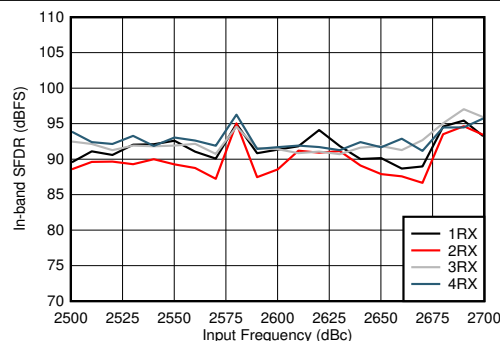
Figure 6-373. RX In-Band SFDR (±200 MHz) vs Frequency With A_{\text{IN}} = -6\text{ dBFS} at 2.6 GHz
