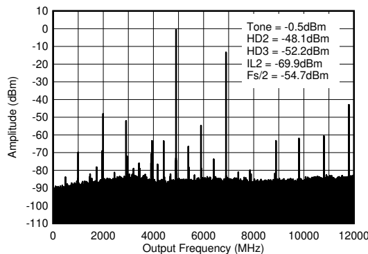
Figure 6-181. TX Single Tone (-12 dBFS) Output Spectrum at 4.9 GHz ( 0-f_{\text{DAC}} )
