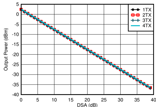
Figure 6-79. TX Output Power vs DSA Setting and Channel at 2.6 GHz
