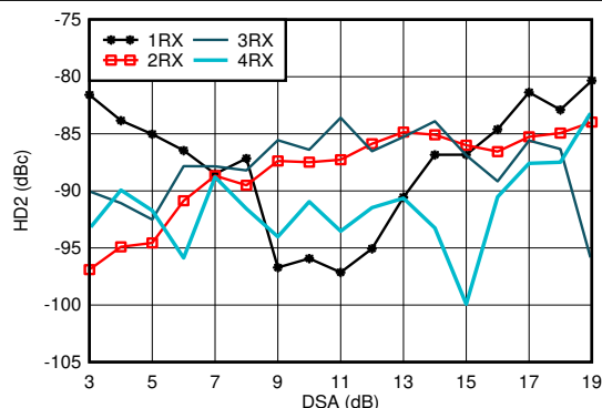
Figure 6-336. RX HD2 vs DSA Setting and Channel at 1.9 GHz
