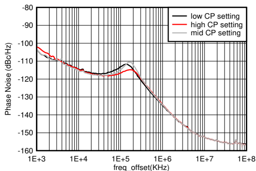
Figure 6-497. Phase Noise for 12-GHz VCO vs Offset Frequency and CP Setting at f_{OUT} = 2.6 GHz
