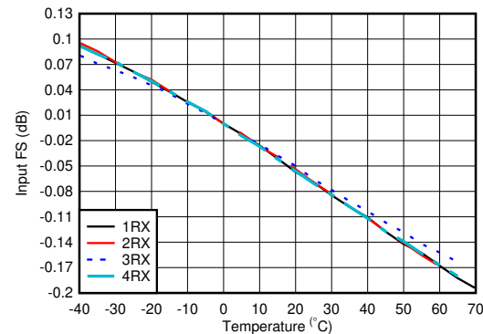
Figure 6-288. RX Input Fullscale vs Temperature and Channel at 800MHz
