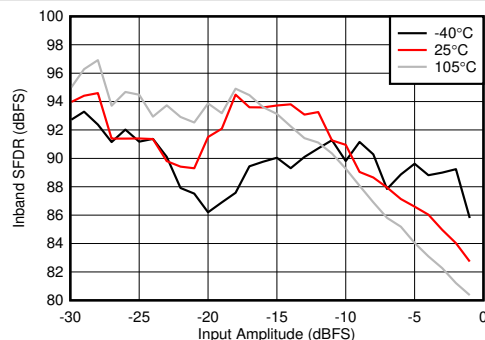
Figure 6-375. RX In-Band SFDR (±200 MHz) vs Input Amplitude at 2.6 GHz
