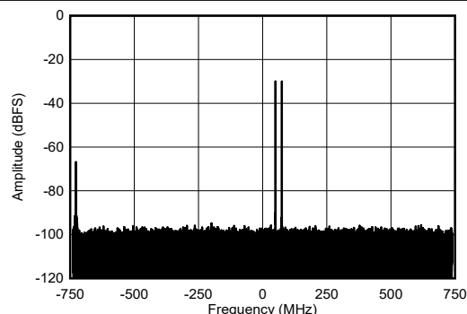
Figure 6-463. RX Dual Tone Output FFT at 8.11GHz
