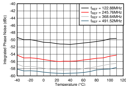
Figure 6-498. Integrated Phase Noise for 12-GHz VCO vs Temperature and f_{REF} at f_{OUT} = 2.6 GHz
