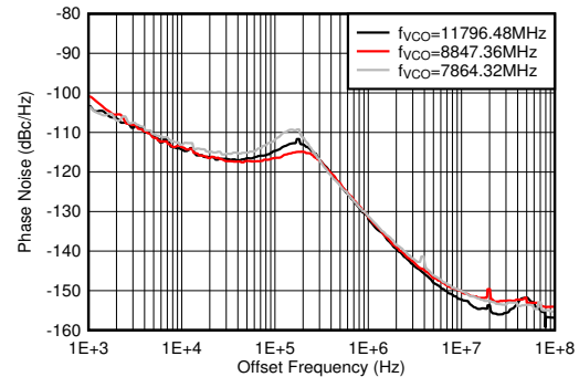
Figure 6-492. Phase Noise vs Offset Frequency and f_{\text{VCO}} at f_{\text{OUT}} = 2610 \text{ MHz}
