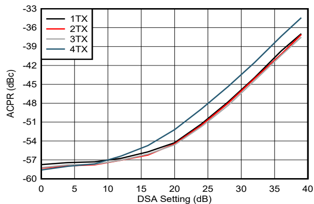
Figure 6-227. TX NR100MHz alt-ACPR vs DSA Setting 8.11 GHz
