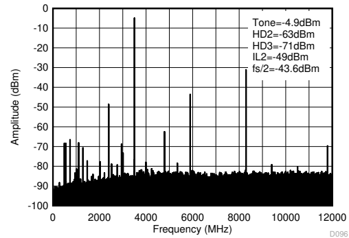
Figure 6-147. TX Single Tone (-6 dBFS) Output Spectrum at 3.5 GHz (0 - f_{\text{DAC}} )
