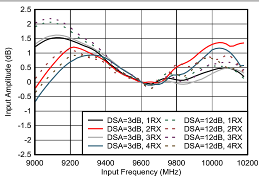
Figure 6-465. RX Input Amplitude vs Frequency
