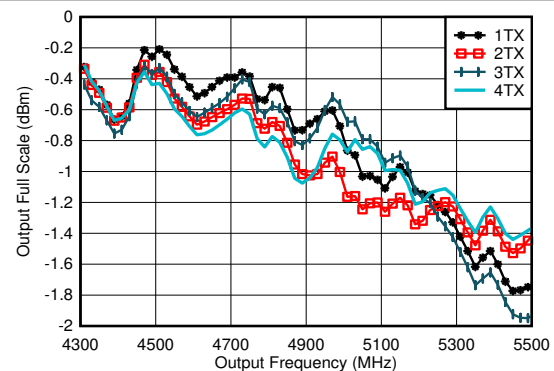
Figure 6-150. TX Full Scale vs RF Frequency and Channel at 5898.24MSPS, Straight Mode, 2nd Nyquist Zone
