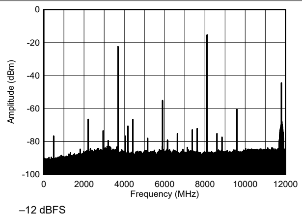
Figure 6-207. TX Single Tone Output Spectrum at 8.11 GHz
