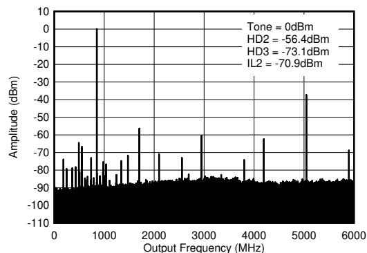
Figure 6-42. TX Single Tone (-6 dBFS) Output Spectrum at 0.85 GHz ( 0-f_{\text{DAC}} )
