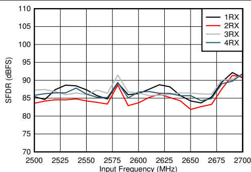
Figure 6-372. RX In-Band SFDR (±200 MHz) vs Frequency With A_{\text{IN}} = -1\text{ dBFS} at 2.6 GHz
