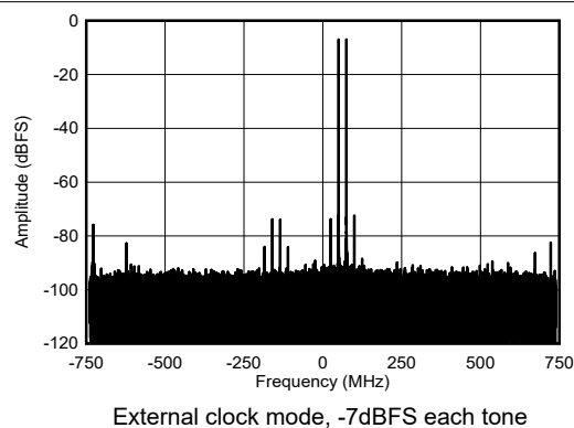
Figure 6-461. RX Dual Tone Output FFT at 8.1GHz
