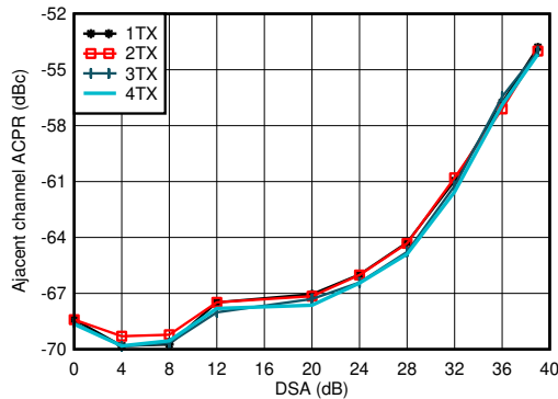
Figure 6-35. TX 20-MHz LTE ACPR vs DSA at 0.85 GHz
