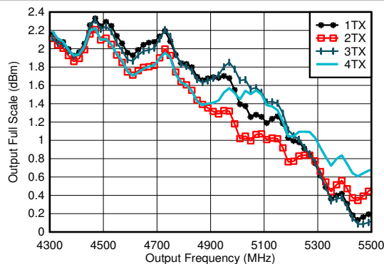
Figure 6-149. TX Full Scale vs RF Frequency and Channel at 11796.48MSPS
