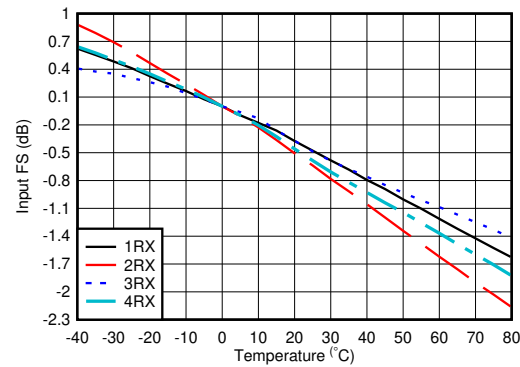
Figure 6-410. RX Input Fullscale vs Temperature and Channel at 4.9 GHz
