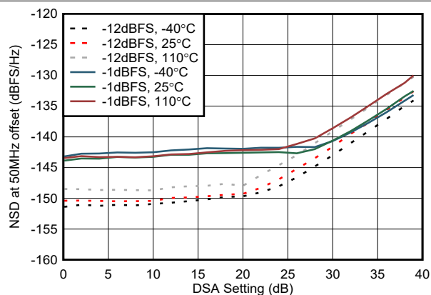
Figure 6-225. TX NSD vs DSA Setting at 8.11 GHz
