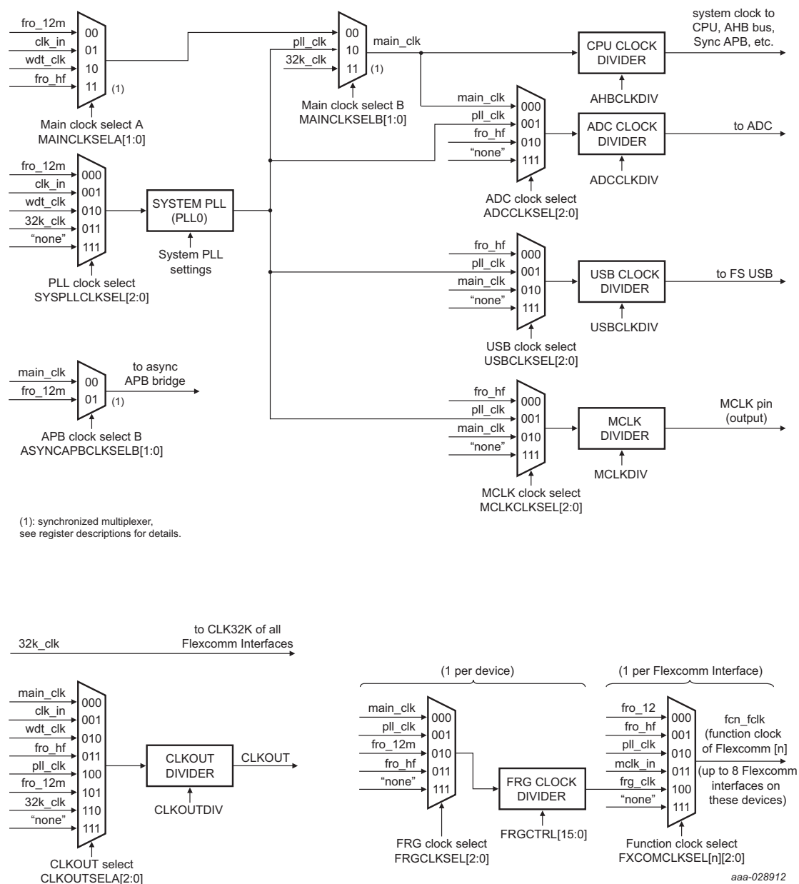
Fig 7. LPC51U68 clock generation
