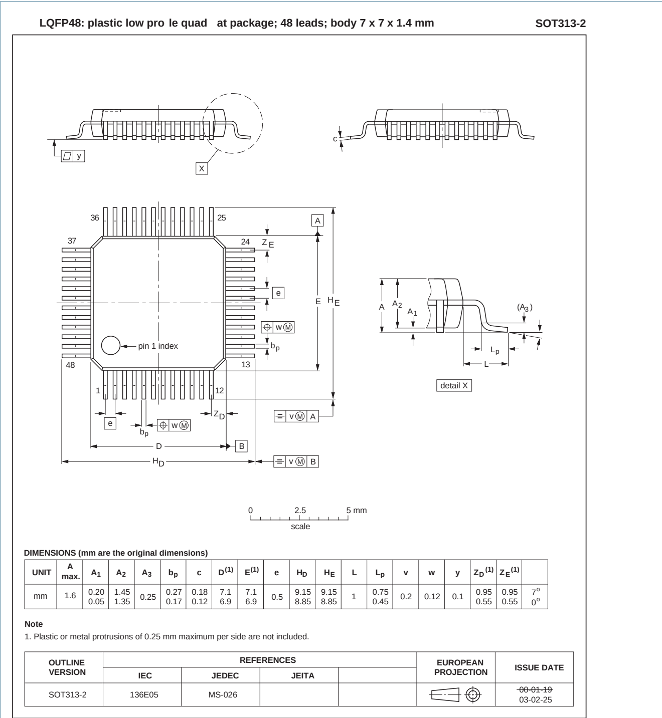
Fig 34. LQFP48 Package outline
