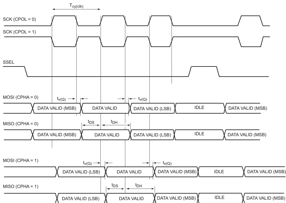
Fig 21. SPI master timing
