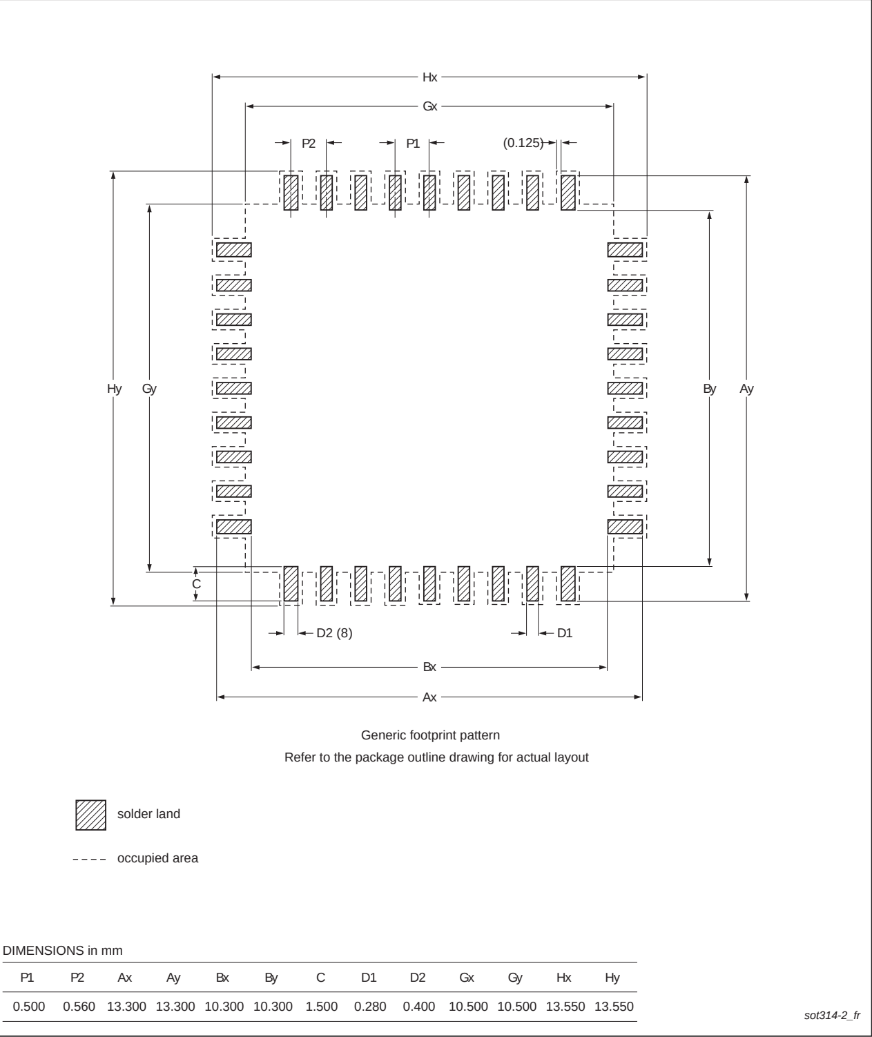
Fig 37. LQFP64 Soldering footprint
