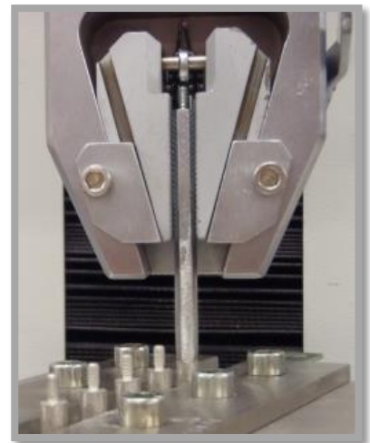
Checking fixture Pull Strength
